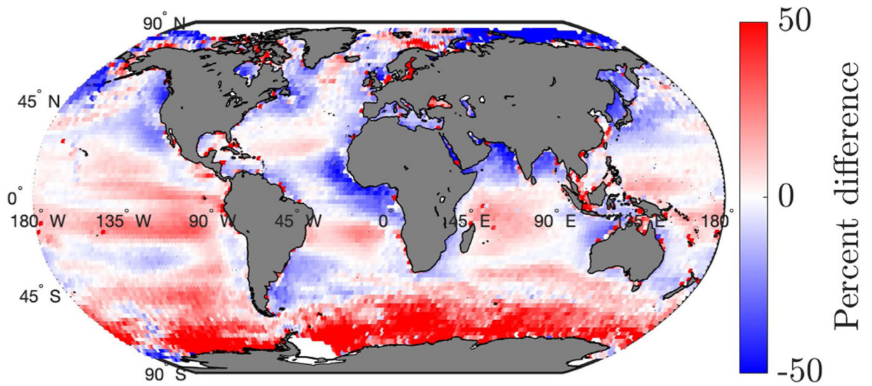
Figure 4. Annually averaged relative percent difference in PhytoC between MODIS and CALIOP, relative to CALIOP (i.e., 100 \times [\text{PhytoC}_M - \text{PhytoC}_C] / \text{PhytoC}_C ). MODIS, Moderate Resolution Imaging Spectroradiometer; CALIOP, Cloud-Aerosol Lidar with Orthogonal Polarization.
