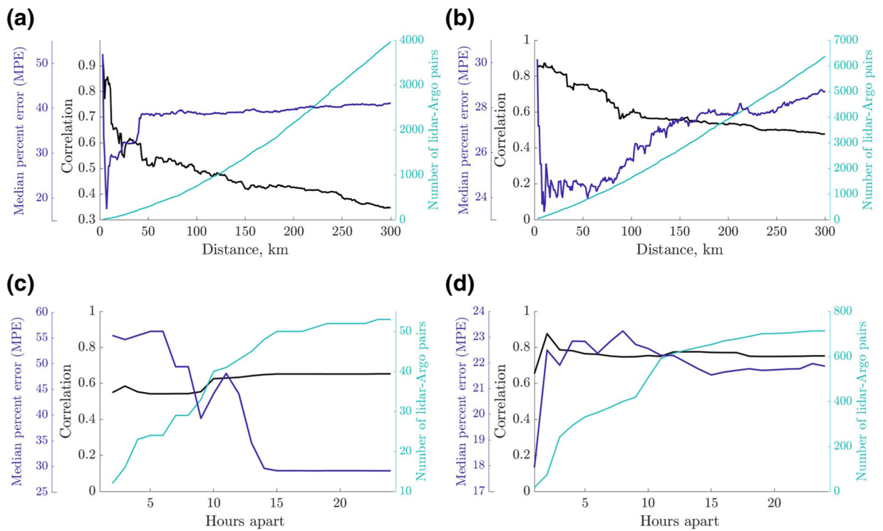
Figure 1. Correlation (black) and median percent error (purple) distances (a, b) and times (c, d) between CALIOP and Argo b_{bp} for areas with mean ocean temperature < and > 15^{\circ}\text{C} (left and right panels, respectively). Cyan lines correspond to the number of observations at a given distance or time. (a, b) Argo and CALIOP are \pm 24 h apart. (c) Argo and CALIOP are 15 km apart. (d) Argo and CALIOP are 50 km apart. CALIOP, Cloud-Aerosol Lidar with Orthogonal Polarization.
