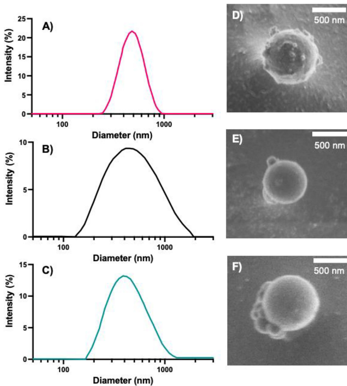
Figure 2: Intensity distribution of A) 0%, B) 10%, and C) 20% NPs acquired from DLS. Representative cryo-SEM images of D) 0%, E) 10%, and F) 20% NPs.
