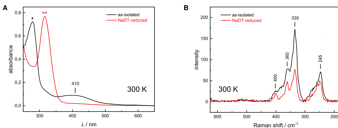
Figure 3. UV/Vis and Raman spectroscopy.
