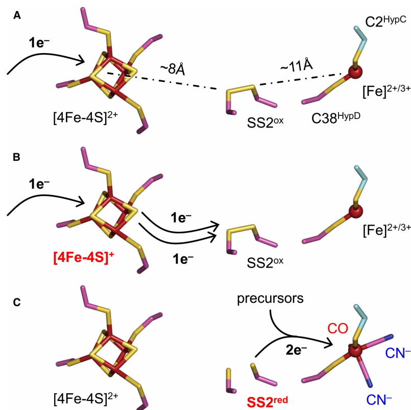
Figure 8. Proposed mechanism for the assembly of the [Fe](CN) 2 CO cofactor precursor.
