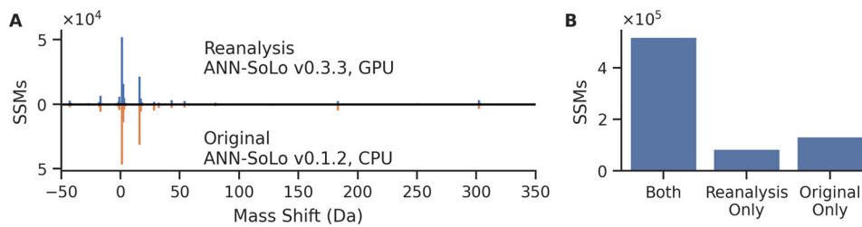
Figure 1: Reanalysis of the Chick et al. [13] HEK293 data with ANN-SoLo. (A) Our reanalysis using ANN-SoLo version 0.3.3 found similar mass shifts for SSMs accepted at 1% FDR when compared to the original analysis [24] conducted with ANN-SoLo version 0.1.2. (B) Although we observed some loss of power, a vast majority of the SSMs from the original analysis were recovered in our reanalysis.
