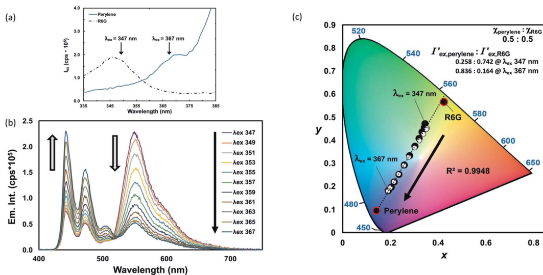
Fig. 4 (a) Overlaid excitation profiles of perylene and R6G in chloroform ( c = 1.2 \times 10^{-6} \text{ M} ) showing the region of interest. (b) Perylene–R6G emission profiles in chloroform ( c = 1.2 \times 10^{-6} \text{ M} ) obtained at various excitation wavelengths (347–367 nm, 2 nm intervals) and (c) the corresponding CIE diagram showing the measured (●) and predicted (○) CIE coordinates. Relative excitation intensities of perylene ( I'_{\text{ex,perylene}} = \frac{I_{\text{ex,perylene}}}{I_{\text{ex,perylene}} + I_{\text{ex,R6G}}} ) and R6G ( I'_{\text{ex,R6G}} = \frac{I_{\text{ex,R6G}}}{I_{\text{ex,perylene}} + I_{\text{ex,R6G}}} ) were calculated using the intensities shown in Table S6, ESI†.
