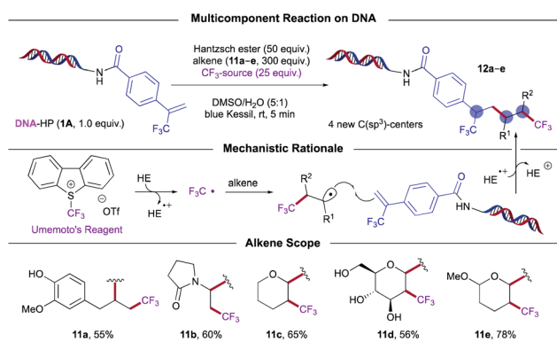
Scheme 6 On-DNA multicomponent trifluoromethylation promoted by photoactive EDA complex activation. Note: several diastereomers are expected to form under these conditions.
