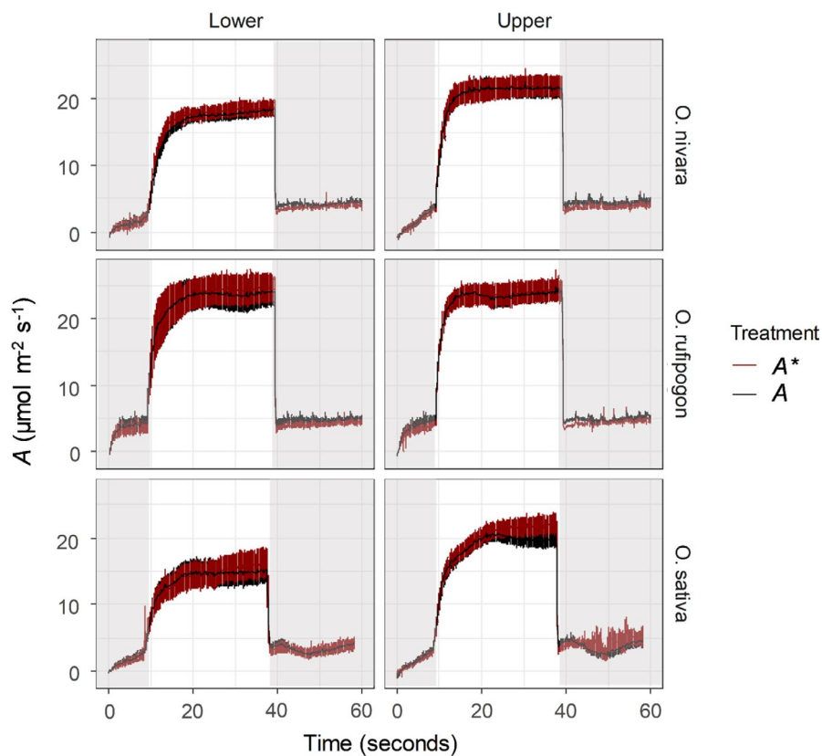
FIGURE 8 The response of uncorrected leaf CO_2 uptake ( A ; ●) and the response of leaf CO_2 uptake corrected for stomatal limitation ( A^* ; ●) over time in different rice species and canopy levels. The vertical line indicates the mean time for the activation of Rubisco ( \tau ) per accession. Each point represents the mean of 6 plants \pm SE ( n = 6 )
