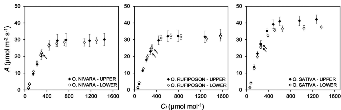
FIGURE 6 Response of CO 2 uptake ( A ) to intercellular [CO 2 ] ( C_i ) in three Oryza species ( O. sativa , O. rufipogon , and O. nivara ) measured at two canopy levels (upper and lower). The CO 2 response curves were measured in saturating light conditions ( 1,500 \mu\text{mol m}^{-2} \text{s}^{-1} ). Each point is the mean ( \pm SE) of six plants ( n = 6 ).
