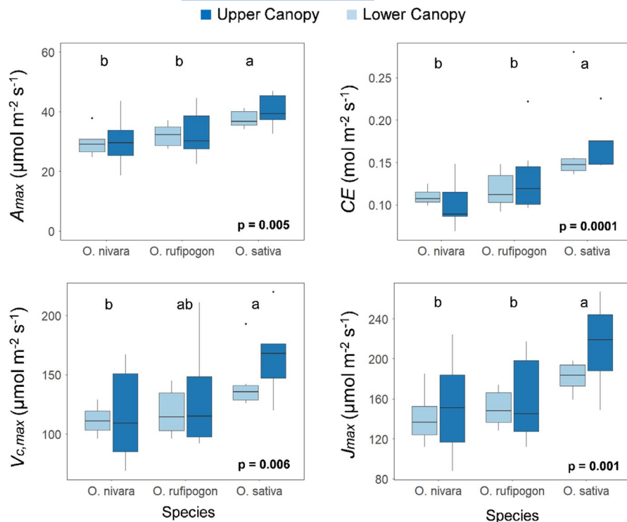
FIGURE 7 Variation for CO_2 uptake in saturating light and [CO_2] ( A_{max} ), carboxylation efficiency ( CE ), the maximum rate of carboxylation efficiency ( V_{c,max} ), and the maximum rate of electron transport ( J_{max} ) in three Oryza species and two canopy levels. Letters are indicative of significant differences between species. Each boxplot represents six plants ( n = 6 )
