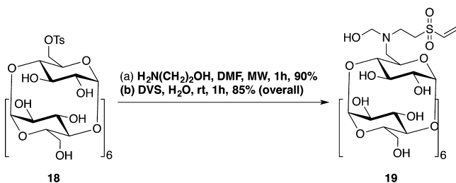
Scheme 3. Synthesis of \beta CD-VS (19) 4a
