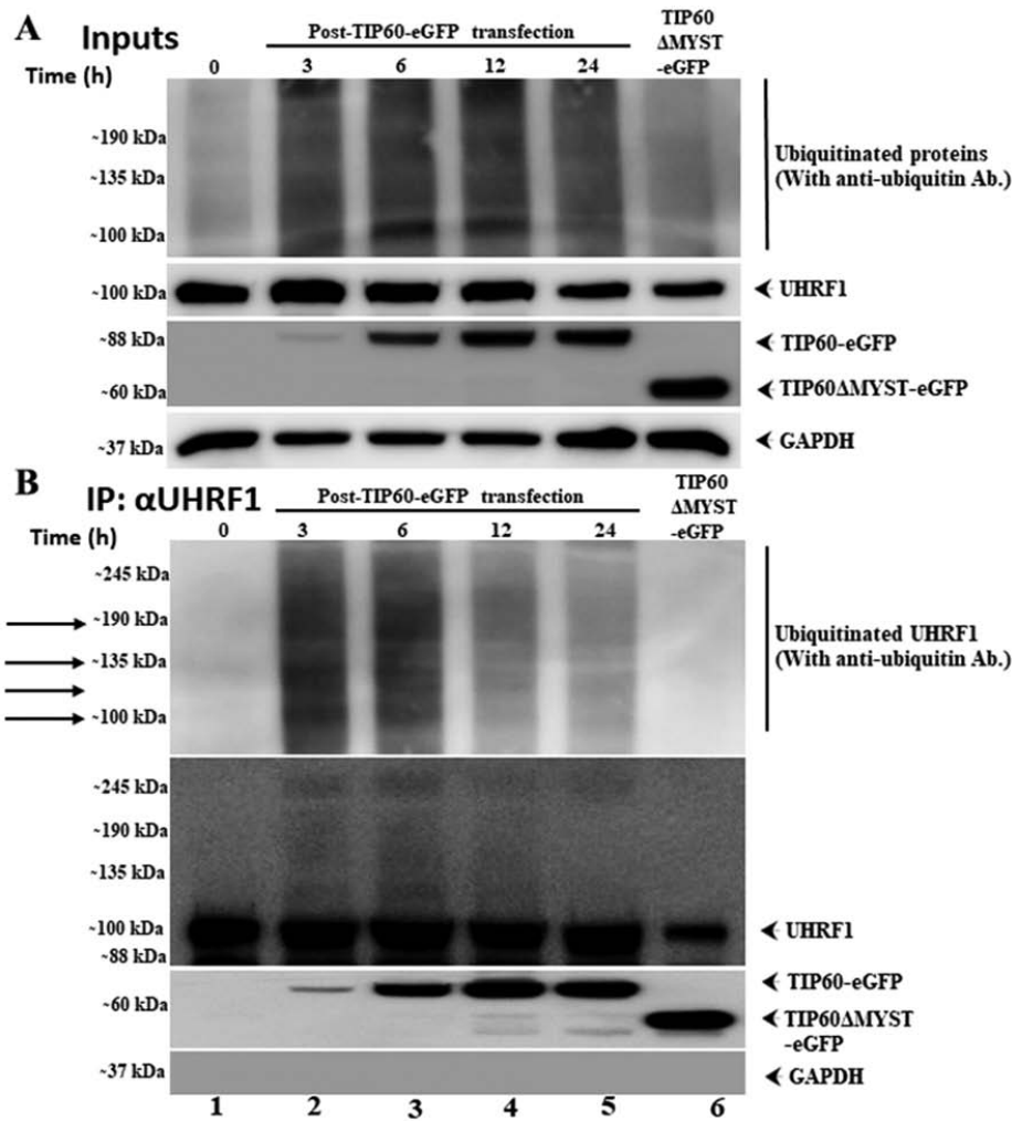
Figure 2. TIP60 induces UHRF1 ubiquitination in HeLa cells. (A and B) Cells were transfected with either TIP60-eGFP WT or TIP60ΔMYST-eGFP mutant. All samples were treated with 10 μM of MG-132 for 8 h before harvesting the cells (In case of 3 and 6 h sample, MG-132 was added 5 and 2 h before transfection, respectively). Cells were collected 3, 6, 12 and 24 h post TIP60 transfection and 24 h in case of TIP60ΔMYST mutant. (A) Represents inputs, while (B) represents immunoprecipitated samples. (B) Immunoprecipitation was performed with anti-UHRF1 antibody. (A) Inputs and (B) immunoprecipitation samples were analyzed by SDS-PAGE and then immunoblotted with anti-UHRF1 and anti-Ubiquitin antibodies. (B) Arrows indicate ubiquitinated UHRF1 bands. Inputs and immunoprecipitation gels were processed in parallel under similar conditions. UHRF1, ubiquitin-like, containing PHD and RING finger domains 1; TIP60, Tat interactive protein, 60 kDa.
