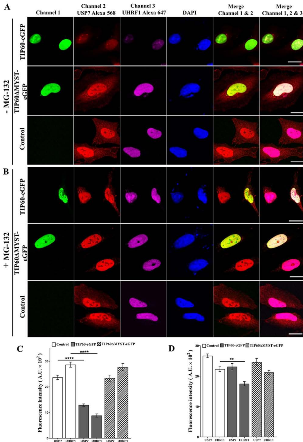
Figure 6. TIP60 downregulates the UHRF1 and USP7 levels in HeLa cells. Cells were either (A) not treated with MG-132 or (B) treated with MG-132 at 10 \mu\text{M} for 8 h. Cells were immunostained with anti-USP7 or anti-UHRF1 antibodies. TIP60-eGFP wild-type (WT) or TIP60ΔMYST-eGFP mutant was transiently overexpressed and their effects were compared with non-transfected control cells. Cells were fixed following transfection and tagged by anti-USP7 and anti-UHRF1 antibodies. Alexa 568 and Alexa 647-labeled secondary antibodies were used as indicated in the figure to visualize the corresponding proteins by confocal microscopy. Scale bar, 10 \mu\text{m} . (C and D) Mean fluorescence intensities representing the levels of USP7 and UHRF1 before and after MG-132 treatment, respectively. Values are the mean \pm SEM for three independent experiments; ** P < 0.01 ; **** P < 0.0001 (vs. control group), determined by one-way ANOVA with Tukey's post hoc test. UHRF1, ubiquitin-like, containing PHD and RING finger domains 1; TIP60, Tat interactive protein, 60 kDa; USP7, ubiquitin-specific-protease 7.
