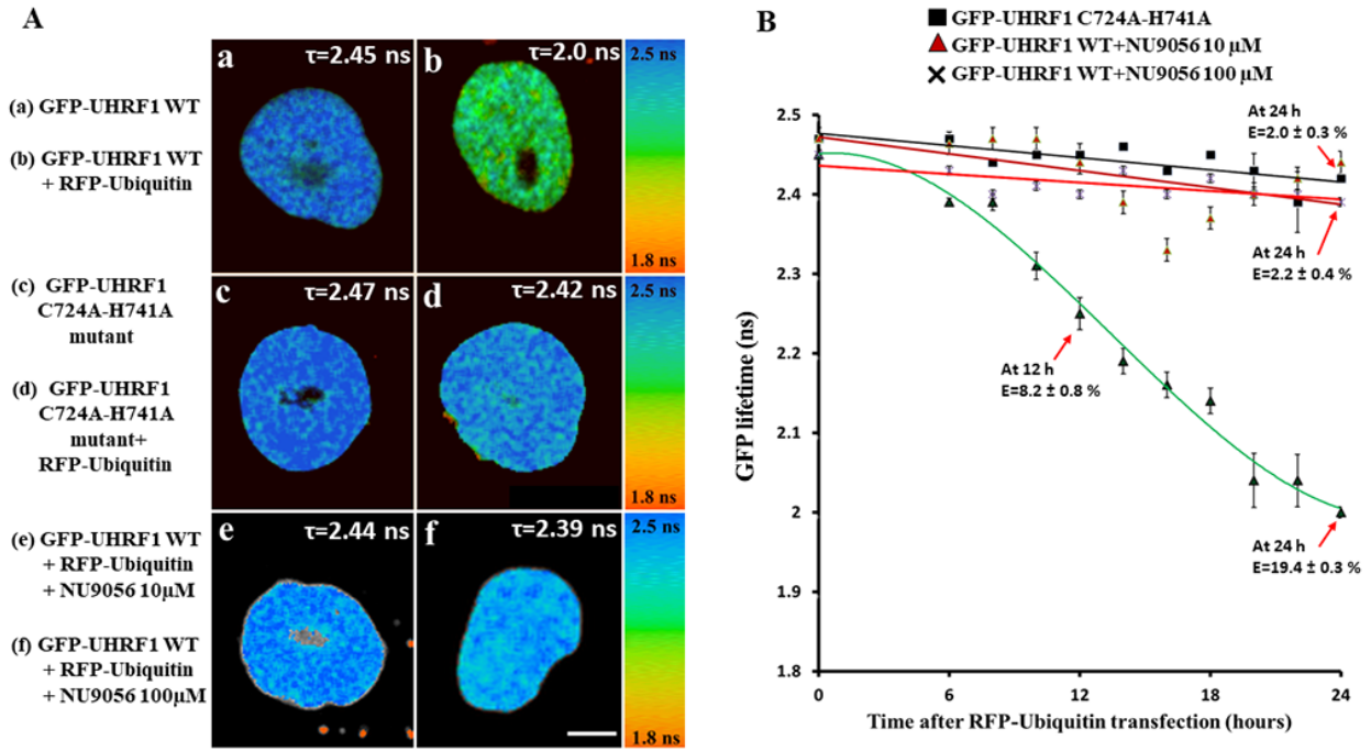
Figure 4. Interaction of UHRF1 and ubiquitin, as determined by FRET-FLIM. (A) Representative 30x30 \mu\text{m} FLIM images of HeLa cells stably expressing (a) GFP-UHRF1 WT and (b) co-transfected with RFP-ubiquitin, HeLa cells (c) stably expressing GFP-UHRF1 C724A-H741A and (d) co-transfected with RFP-ubiquitin. The lifetime values are shown by a color code ranging from red (1.8 ns) to blue (2.5 ns). Scale bar, 10 \mu\text{m} . In comparison to cells (a) expressing only GFP-UHRF1 WT, a marked decrease in the GFP lifetime and thus, a strong FRET efficiency was observed when HeLa cells were (b) transfected with RFP-ubiquitin. By contrast, no substantial difference in lifetime or FRET efficiency was observed when HeLa cells expressing GFP-UHRF1 C724A-H741A were transfected with RFP-ubiquitin (compare panels d and c). No difference in lifetime or FRET efficiency was observed in HeLa cells expressing GFP-UHRF1 WT in the presence of the TIP60 inhibitor NU9056 (e) 10 \mu\text{M} or (f) 100 \mu\text{M} . FLIM data indicate that UHRF1 interacts with ubiquitin while this interaction is impaired in case of UHRF1 having a RING finger domain mutation. (B) Change in GFP lifetime as a function of time. Values are the mean \pm SEM from three independent experiments. The fluorescence lifetimes of GFP-UHRF1 WT (without and with TIP60 inhibitor NU9056 10 \mu\text{M} , 100 \mu\text{M} ) or GFP-UHRF1 C724A-H741A were measured at different times following transfection with RFP-Ubiquitin. FRET efficiency was calculated according to E=1-(\tau_{DA}/\tau_D) , where \tau_{DA} is the lifetime of the donor (GFP) in the presence of acceptor (RFP) and \tau_D is the lifetime of GFP in the absence of acceptor. UHRF1, ubiquitin-like, containing PHD and RING finger domains 1; TIP60, Tat interactive protein, 60 kDa.
