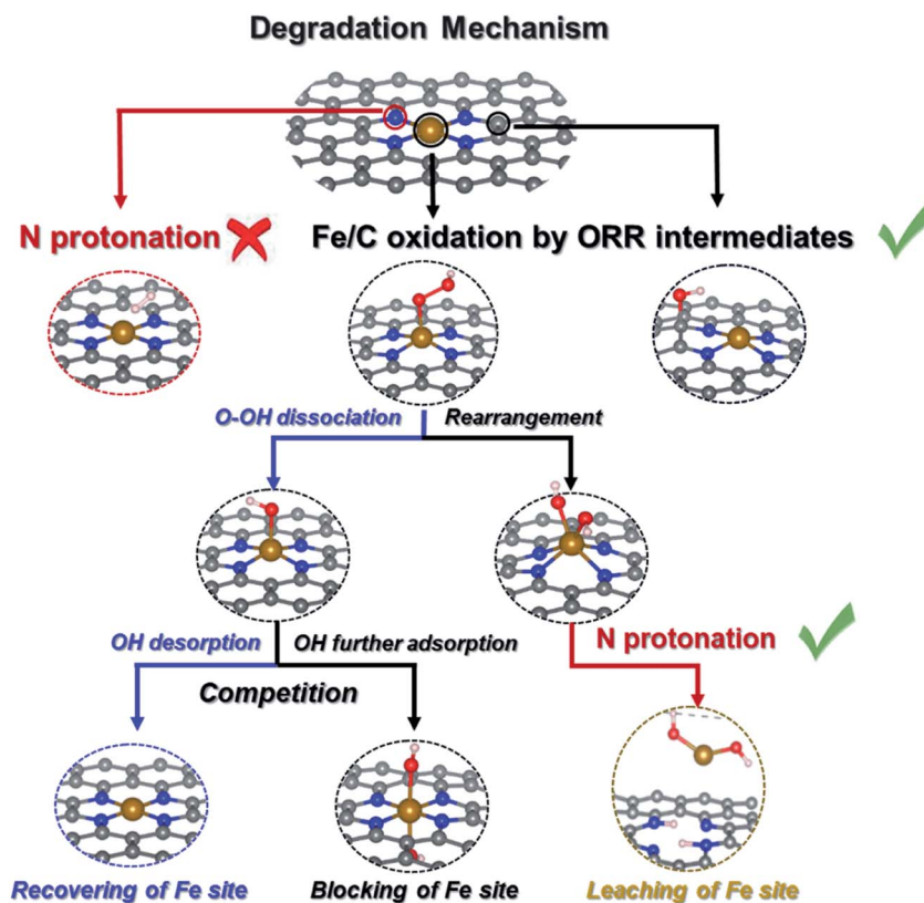
Scheme 2 The pathway of the degradation mechanism of an FeNC catalyst.
