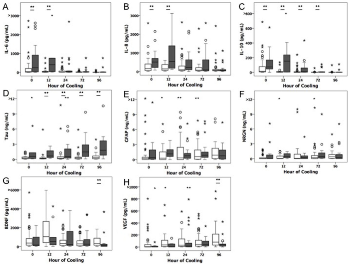
Fig 1. Box plots depicting medians and interquartile ranges of raw biomarker data over time. Data from infants who died or had severe brain injury by MRI (gray boxes) are compared to those who survived with normal or mild injury by MRI. Outliers and extremes represented by open circles and asterisks respectively. § denotes significance (P<0.05) by logistic regression analyses.
