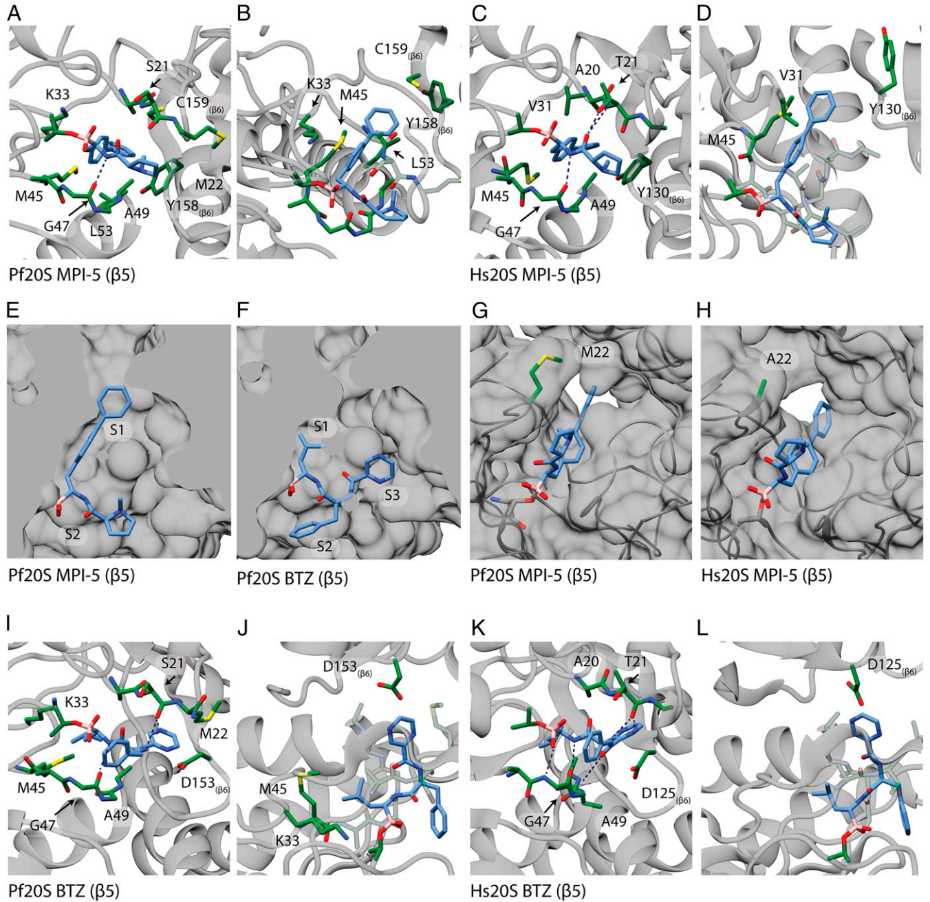
Fig. 3. Structures of Pf 20S and Hs 20S \beta 5 active sites with bound MPI-5 or bortezomib. Pf 20S \beta 5 (A and B) and Hs 20S \beta 5 c (C and D) are shown as side (A and C) and top (B and D) views, with interacting residues (green) around the covalently bound MPI-5 (blue). (E and F) Cut-away showing solvent-accessible surface of the Pf 20S \beta 5 active site illustrating the different poses adopted by MPI-5 (E) and bortezomib (F). Substrate binding pockets, S1, S2, and S3 are marked. (G and H) Met22 creates a hydrophobic ledge over the ligand binding site in Pf 20S \beta 5 , while Ala22 permits more solvent access in the Hs 20S \beta 5 c active site around the covalently bound MPI-5. Pf 20S \beta 5 (I and J) and Hs 20S \beta 5 c (K and L) are shown as side (I and K) and top (J and L) views, with interacting residues (green) around the covalently bound bortezomib (blue).
