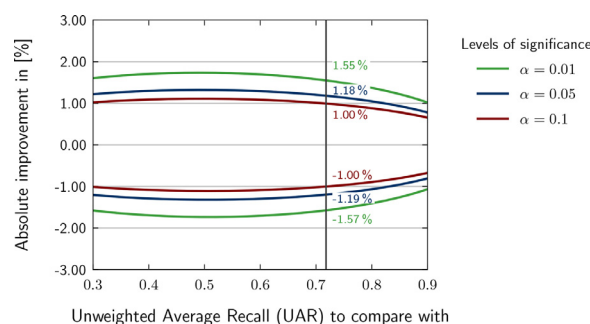
Fig. 6. Two-sided significance test on the MSC Test set with various levels of significance.
