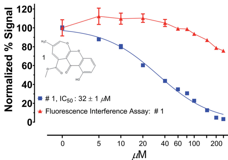
Fig. 4. Fluorescence interference assay. Compound 1 was isolated from a fluorescence based protease inhibitor assay and was then rescreened in dose response against the fluorophore alone (7-aminomethylcoumarin) and found not to interfere with fluorescence detection throughout the IC 50 range of compound 1 . Reprinted with permission from: T. D. Tran, B. A. P. Wilson, C. J. Henrich, L. M. Staudt, L. R. H. Krumpke, E. A. Smith, J. King, K. L. Wendt, A. M. Stchigel, A. N. Miller, R. H. Cichewicz, B. R. O'keefe and K. R. Gustafson, J. Nat. Prod. , 2019, 82 , 154–162. Copyright 2019 American Chemical Society.
