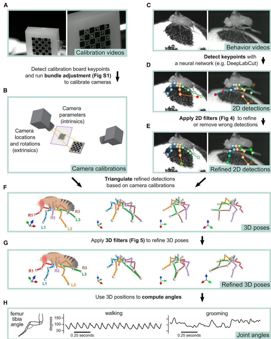
Figure 2. Overview of the Anipose 3D tracking pipeline
