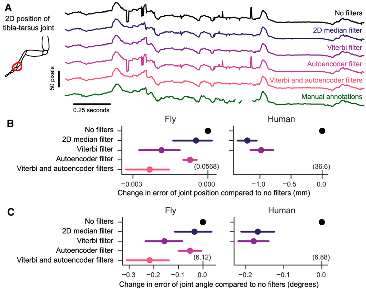
Figure 4. 2D filters improve accuracy of 2D pose estimation by taking advantage of the temporal structure of animal behavior
