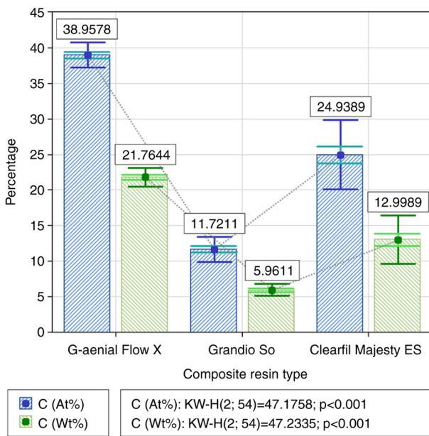
Figure 1. Statistical analysis of the mass (Wt%) and atomic percentage (At%) of the carbon (C) content for the three types of materials.
