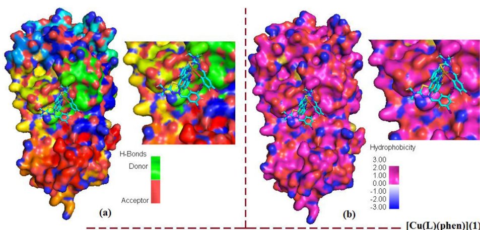
Fig. 8. The total density surfaces representation for docked copper (II) complex [Cu(L)(phen)](1) inside the M Pro protein (PDB ID: 7C8U) (a) with hydrogen bond donor and acceptor meshes represented by light green and red colors, respectively (b) Surface representation of hydrophobic pocket represented with dee pink and light blue colors (For interpretation of the references to color in this figure legend, the reader is referred to the web version of this article.).
