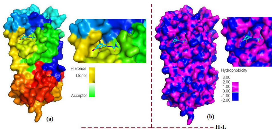
Fig. 7. The total density surfaces representation for docked Schiff base ligand (H 2 L) inside the M Pro protein (PDB ID: 7C8U) (a) with hydrogen bond donor and acceptor meshes represented by yellow and green colors, respectively (b) Surface representation of hydrophobic pocket represented with pink and blue colors (For interpretation of the references to color in this figure legend, the reader is referred to the web version of this article.).
