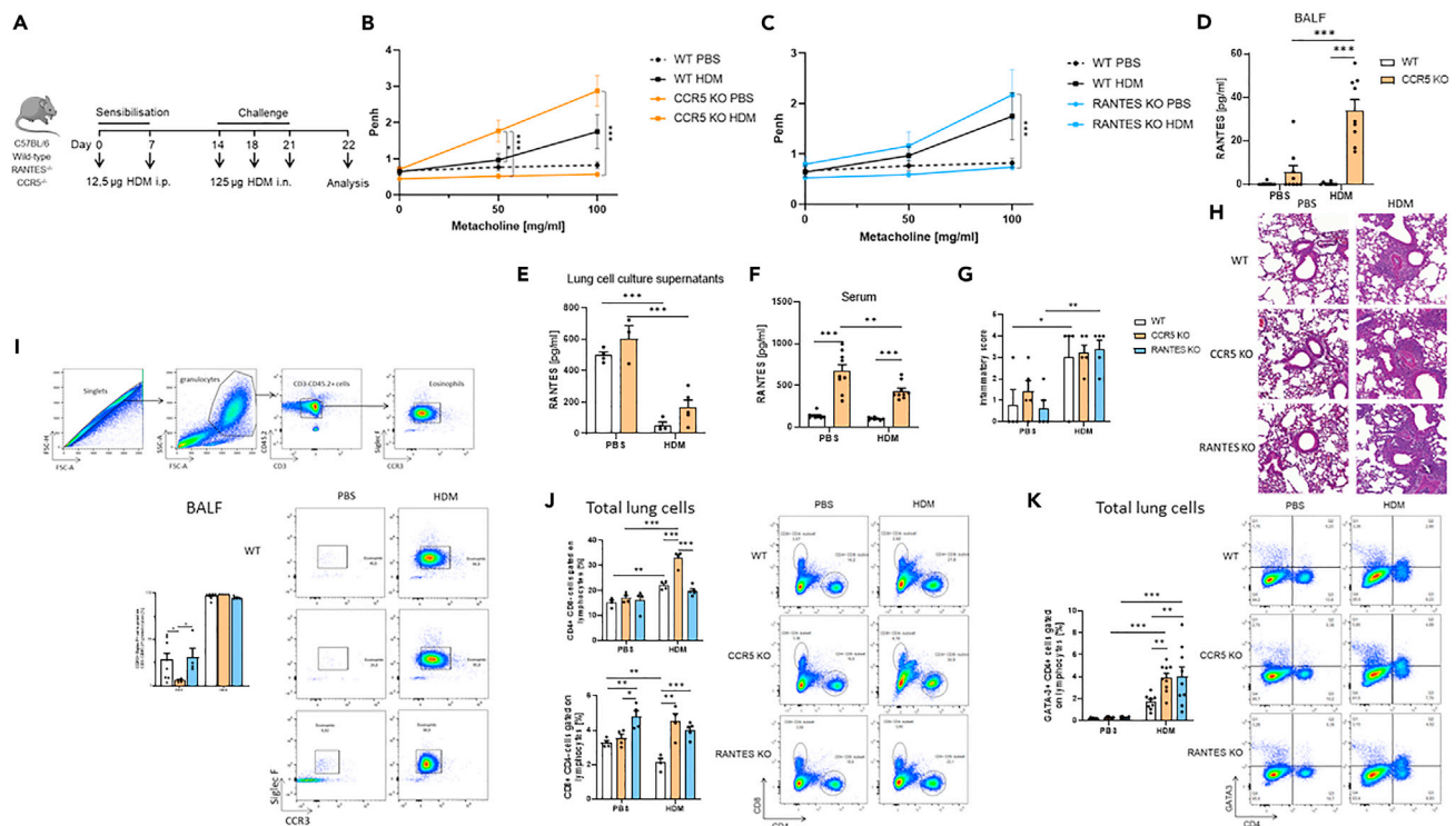
Figure 4. RANTES -/- and CCR5 -/- mice have more eosinophils in the airways and a higher percentage of Th2 cells in the lung (A) Experimental design of the murine asthma model. (B and C) Lung function measured by Buxco system in response to increasing doses of methacholine. (D, E, and F) RANTES was measured in BALF (D), re-stimulated lung cell supernatants (E), and serum (F) by ELISA. (G and H) Representative hematoxylin and eosin-stained sections of the lung and respective inflammatory score. Scale bar, 150 \mu m. (I) Flow cytometry analysis and representative dot plots of the CCR3+ Siglec F+ eosinophils gated on CD3- CD45.2+ granulocytes in the bronchoalveolar lavage. (J) Flow cytometry analysis and representative dot plots of the CD4+ CD8- and CD8+ CD4- cells gated on lymphocytes in the lung. (K) Flow cytometry analysis and representative dot plots of the GATA3+ CD4+ cells gated on lymphocytes in the lung. Data are shown as mean values \pm SEM with n = 3–5 per group (B, C, E, I, and J) or n = 8–9 with data pooled from two independent experiments (n = 3–5 per group; D, F, and K), each symbol representing individual mice. p Values were calculated using two-way analysis of variance. *p, 0.05; **p, 0.01, ***p, 0.001. See also Figures S2 and S3.
