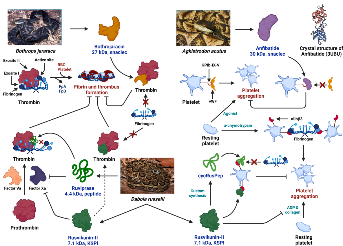
Fig. 4. Antithrombotic mechanisms of Bothrojaracin, Anfibatide, Ruvikunin-II and Ruviprase. Bothrojaracin binds to exosite I of thrombin and interferes with the binding of fibrinogen to thrombin. Consequently, fibrinogen is not accessible to thrombin for catalysis and fibrin clot formation is inhibited. Anfibatide binds to the GPIb-IX-V platelet receptor and inhibits the association of vWF with this platelet receptor which subsequently inhibits platelet aggregation. Ruviprase and Ruvikunin II exhibit dual inhibition of thrombin and factor Xa. While Ruviprase binds to the active site of thrombin, Ruvikunin II occupies thrombin exosite I and inhibits the conversion of fibrinogen to fibrin. In addition, the synthetic peptide cycRusPep derived from Ruvikunin II binds to the \alpha IIb \beta 3 receptor and inhibits platelet aggregation mediated by the association of fibrinogen to this receptor.
