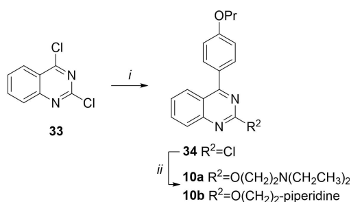
Scheme 3. Reagents and condition: i ) 4-propoxyphenylboronic acid, \text{Pd}(\text{PPh}_3)_4 , DME, aq. 2 M \text{Na}_2\text{CO}_3 , MW, 100^\circ\text{C} , 15 min, 72%; ii ) 2-(diethylamino)ethan-1-ol or 1-piperidinethanol, NaH, dry THF, reflux, 1 h, 50–55%.
