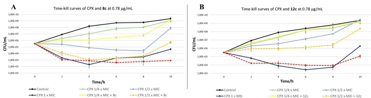
Figure 5. Time-kill curves of CPX at \frac{1}{4} , \frac{1}{2} and 1 \times MIC alone or in combination with compound 8c (A) and 12c (B) at 0.78 \mu g/mL against S. aureus strain SA-1199B. Assays were performed testing at each time points 4 dilutions in duplicate.
