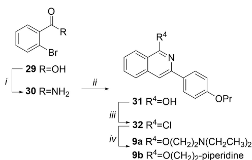
Scheme 2. Reagents and condition: i ) a) \text{SOCl}_2 , reflux, 1 h; b) aq. 33% \text{NH}_3 , \text{CH}_3\text{CN} , rt, 1 h, 95%; ii ) \text{CuBr} , 1-(4-propoxyphenyl)ethan-1-one, \text{Cs}_2\text{CO}_3 , dry DMSO, 110^\circ\text{C} , 8 h, 30%; iii ) \text{POCl}_3 , reflux, 3 h; iv ) 2-(diethylamino)ethan-1-ol or 1-piperidinethanol, NaH, dry THF, reflux, 1–3 h, 50–53%.
