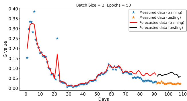
Fig. 6. Comparison between predicted and measured G values, using simple DNN model, for 25 Jan 2020 to 11 May 2020 using TfidfVectorizer pre-processing model with fixed vector size of 94,237.
