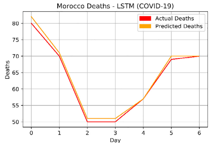
Fig. 18. Morocco Deaths (LSTM).
