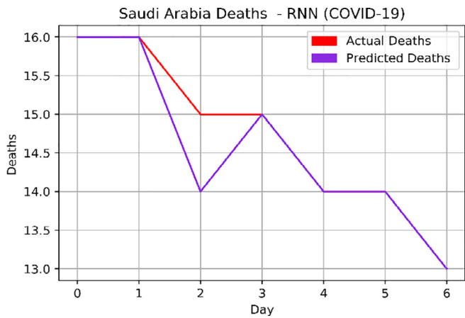
Fig. 9. Saudi Arabia Deaths (RNN).
