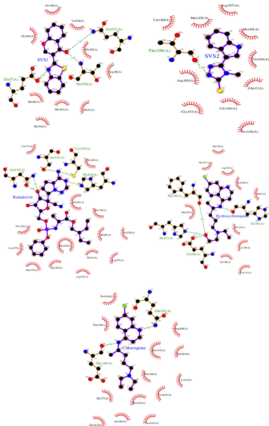
Fig. 8. Ligplot image showing the hydrogen bonds (green dashed lines) and hydrophobic interactions (red arcs) of the compounds ( SVS1 , SVS2 , remdesivir, hydroxychloroquine and chloroquine) at the active site of SARS-CoV-2 main protease enzyme (6Y2F).
