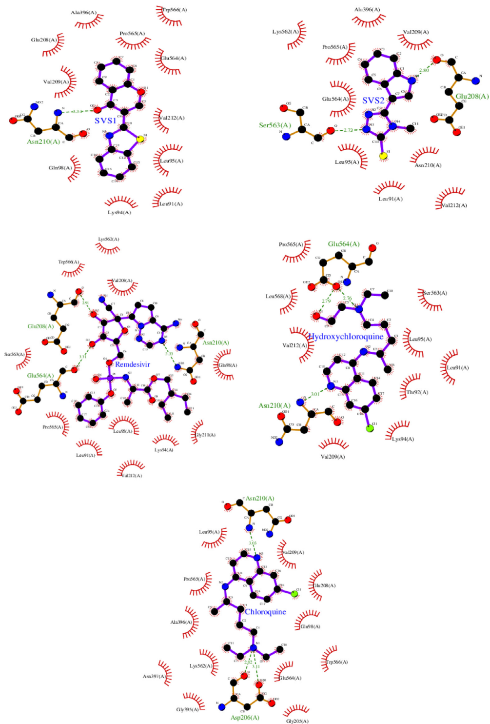
Fig. 9. Ligplot image showing the hydrogen bonds (green dashed lines) and hydrophobic interactions (red arcs) of the compounds (SVS1, SVS2, remdesivir, hydroxychloroquine and chloroquine) at the active site of human ACE-2 enzyme (6M0J).
