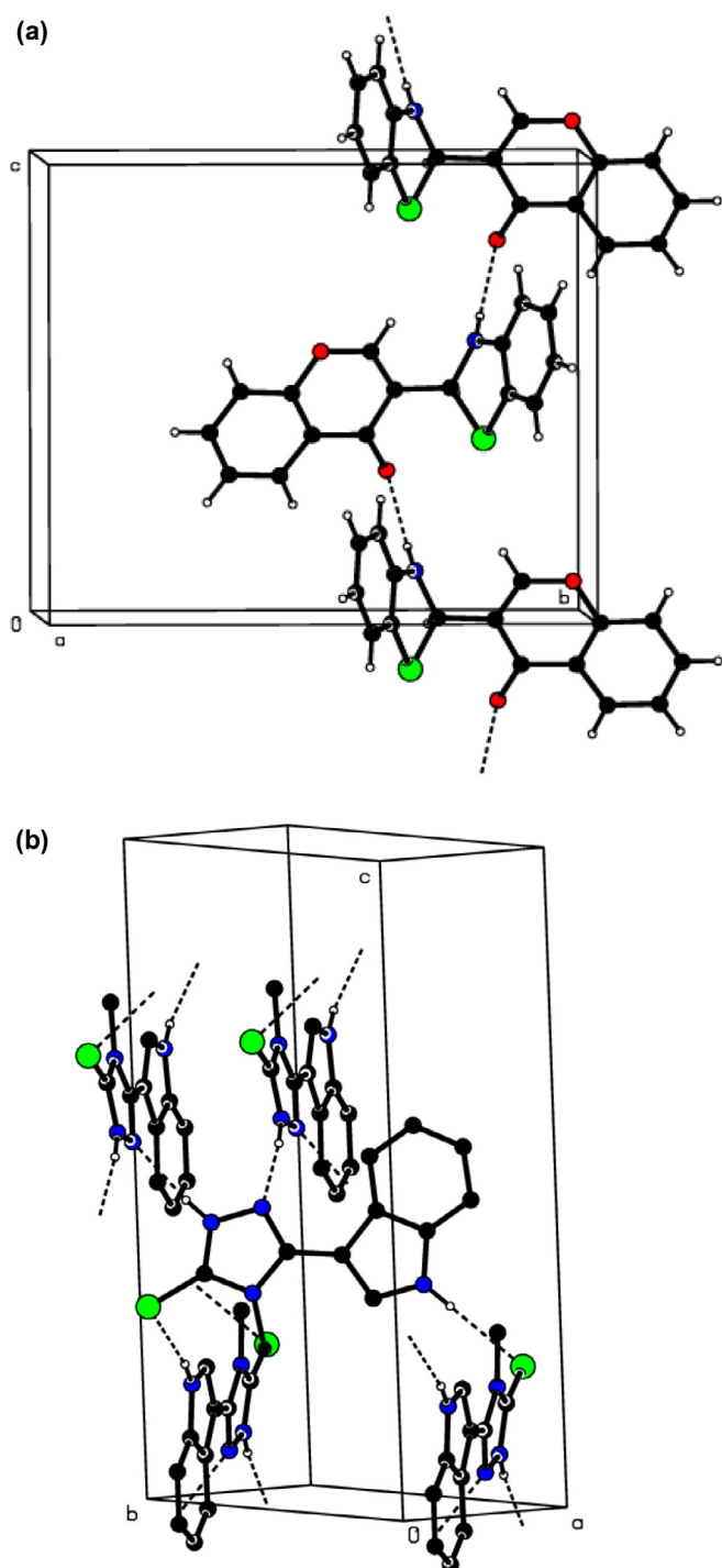
Fig. 4. Packing diagram showing inter-molecular hydrogen bonding interactions in (a) SVS1 and (b) SVS2 .
