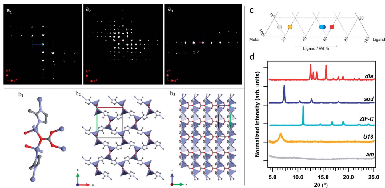
Fig. 2 2D slice cuts from the reconstructed 3D reciprocal lattice show the 0kl ( a_1 ), hk0 ( a_2 ) and h0l ( a_3 ) planes. The scattering background (see Fig. S2†) was removed for clarification. Structure of ZIF-CO3-1: ( b_1 ) coordination mode of Zn; ( b_2 ) framework viewed along the c axis; ( b_3 ) framework structure viewed along the a axis. The Zn, O, N and C atoms are shown in blue, red, light blue and grey, respectively. (c) Section of the ternary diagram to highlight the samples selected as representative of the different phases (grey spot: amorphous biocomposite (TD- \text{H}_2\text{O} ); yellow spot: U13 (TD- \text{H}_2\text{O} ); azure: ZIF-C (TD- \text{H}_2\text{O} ); blue: sod (TD-EtOH); red: dia (TD-EtOH)). The ZIF-C and sod samples were obtained with the same protocol, but with different washing procedures (TD- \text{H}_2\text{O} and TD-EtOH, respectively). (d) XRD patterns of the amorphous biocomposite and of the biocomposites with dia , sod , ZIF-C topologies, and U13 .
