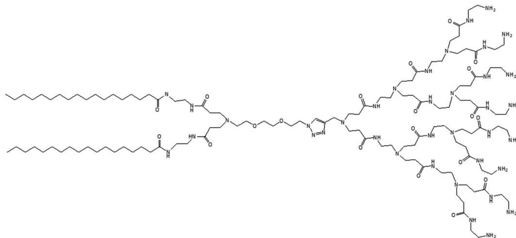
Fig. 13 Chemical structure of lipid-modified amphiphilic PAMAM dendrimer (AD) obtained by conjugating two precursors (azide-functionalized hydrophilic dendrimer moiety and alkyne-functionalized C-18 alkyl bearing hydrophobic moiety) through click chemistry.
