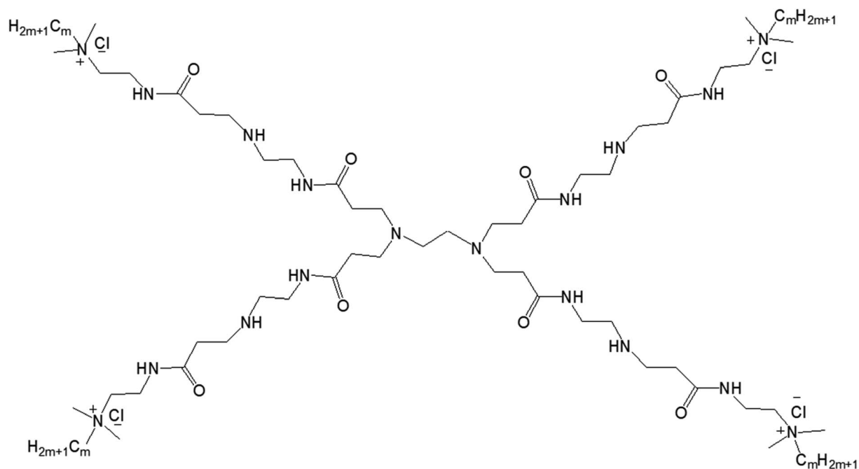
Fig. 14 Chemical structure of amphiphilic lipid-modified PAMAM dendrimers G_nQPAMC_m (where n = 1 (dendrimer generation) and m = 8, 12, 16 (alkyl chain length after the modification of the end group)).
