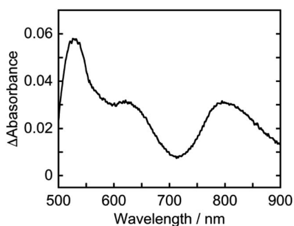
Fig. 7 Difference absorption spectrum from before and after electrocatalytic one-electron reduction of Os. A CO 2 -saturated DMA solution containing Os (0.5 mM) and Et 4 NBF 4 (0.1 M) as an electrolyte was reduced at -1.75 V using a UV-vis OTTLE cell with a Pt mesh working electrode and Ag/AgNO 3 reference electrode.
