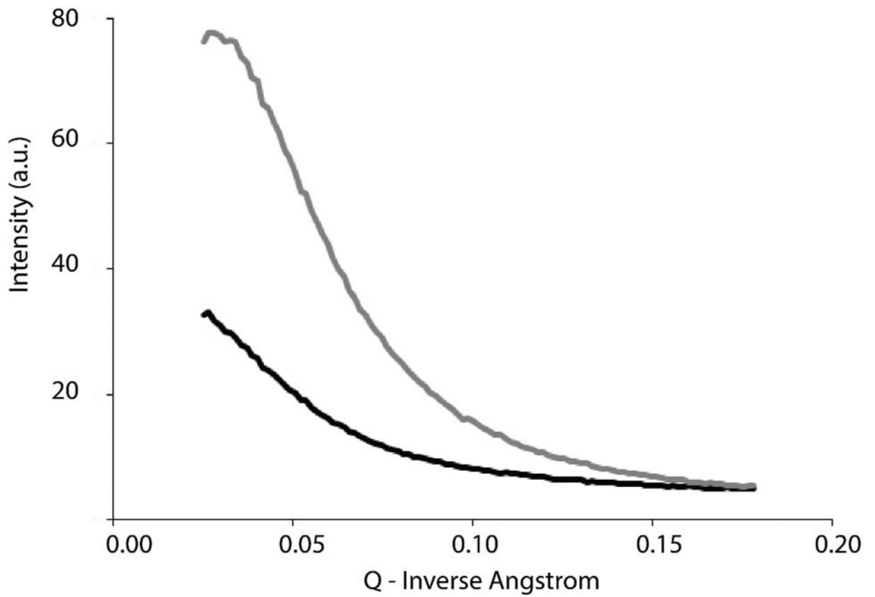
Figure 2. Small angle x-ray scattering (SAXS) of films. Black line) Alginate and GMHA films without urea crystal templating. Gray line) Alginate and GMHA films with urea crystal templating.
