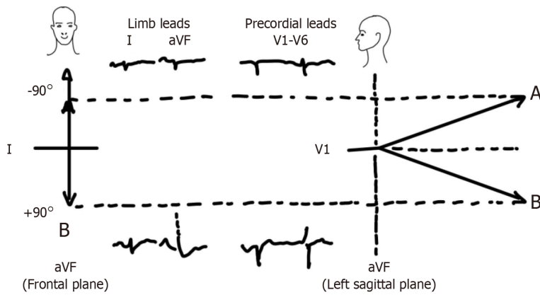
Figure 8 This is a schematic illustration of the axis-illusion phenomenon. A and B are frontal mean QRS axes of -90^\circ and +90^\circ respectively, suggesting a 180^\circ divergence. Their sagittal projections reveal that this is illusory since they are actually much closer in space. Concept adapted from David Spodick's work.
