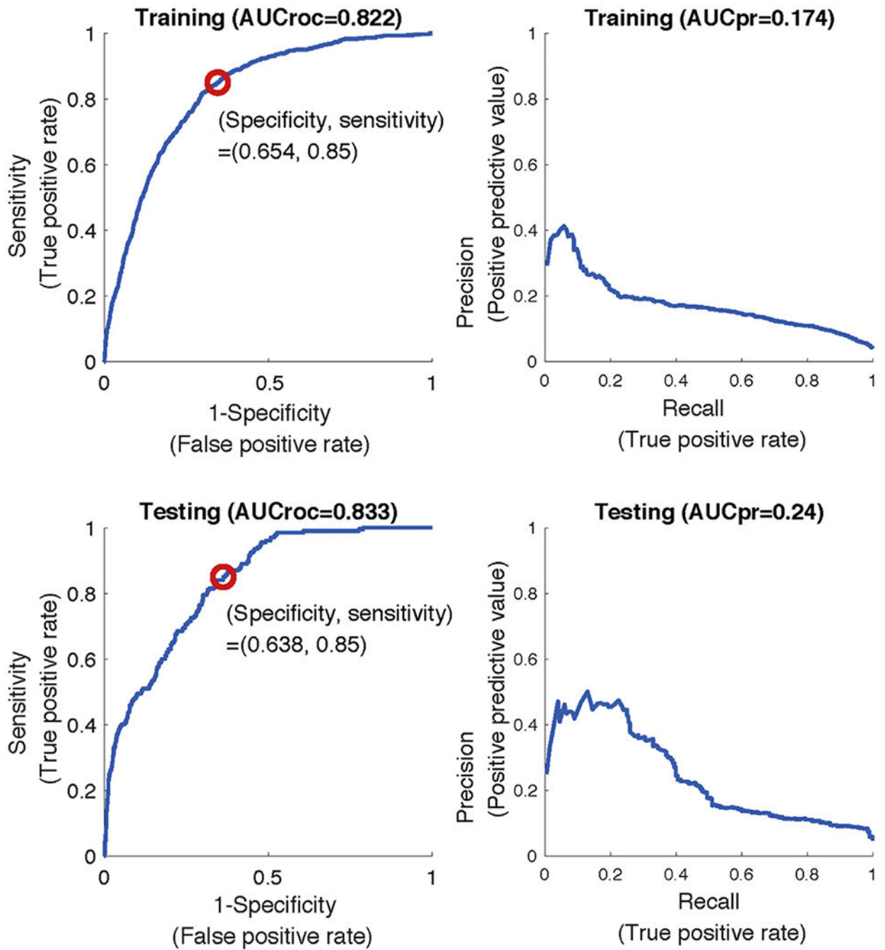
Figure 4. AUC ROC and precision-recall curves for predicting t-sepsis 12 hours in advance at the development site using CMS severe sepsis definition. AUCroc , Area under the receiver operating characteristic; AUCpr , AUC precision-recall curve.
