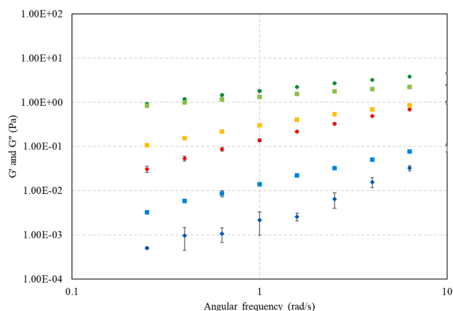
Fig. 4. Rheological characterisation of the viscoelastic XG systems. Storage modulus G' for 0.1% ( \square ), 0.3% ( \square ) and 0.5% ( \square ) XG, and loss modulus G'' for 0.1% ( \square ), 0.3% ( \square ) and 0.5% ( \square ) XG as a function of the angular frequency. Error bars indicate the standard deviation.
