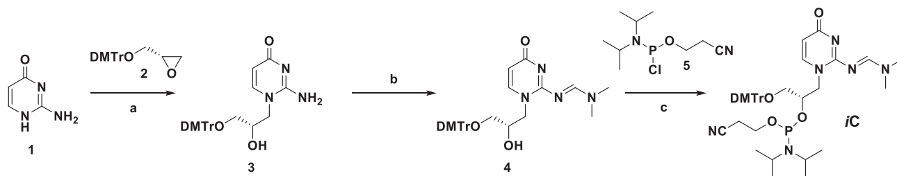
Scheme 1. Synthesis of ( S )-GNA-isocytidine phosphoramidite iC . (a) NaH, DMF, 43%; (b) DMF-DMA, MeOH, 96%; (c) DIPEA, CH 2 Cl 2 , 32%. DMF-DMA = N,N -dimethylformamide dimethylacetal; DIPEA = N,N -diisopropylethylamine.
