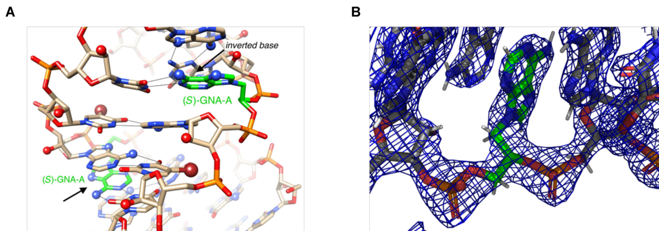
Figure 3. The RNA dodecamer duplex with single ( S )-GNA-A residues (carbon atoms colored in green) viewed into the central minor groove. (A) The inverted orientation of GNA residues is indicated with arrows and all adenine N6 and N7 (blue), 2'-hydroxyl oxygen (red), and bromine atoms (brown) are highlighted in ball-and-stick mode. H-bonds are drawn with thin lines. (B) F_{\text{obs}} - F_{\text{calc}} electron density of the ( S )-GNA-A residue demonstrating the unambiguous orientation of the nucleobase.
