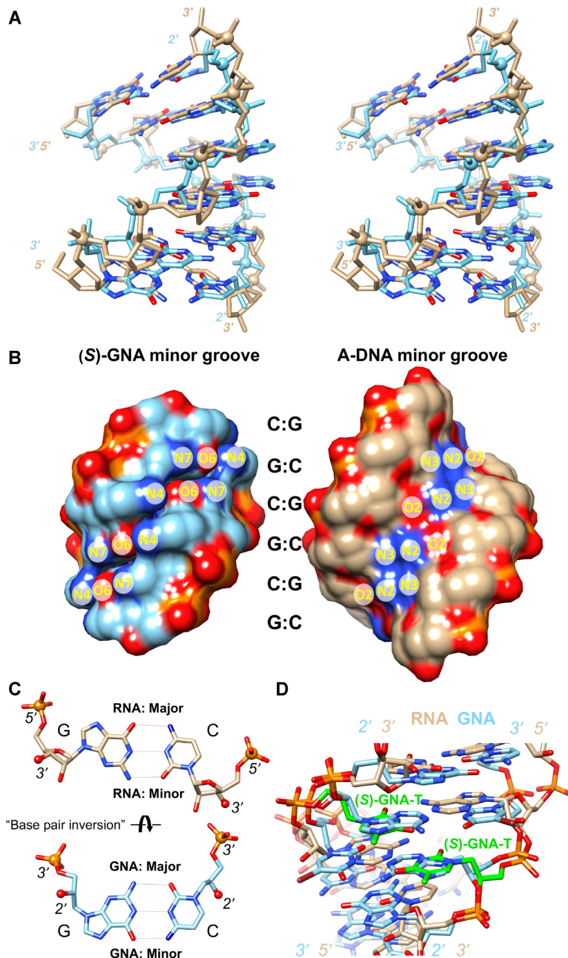
Figure 2. GNA displays an inverted base pair orientation relative to DNA and RNA. (A) Cross-eye stereo image of the (S)-GNA hexamer duplex (20) with sequence 3'-GCGCGC-2' (light blue, PDB ID 2WNA) superimposed on the A-DNA model duplex with sequence 5'-GCGCGC-3' (tan). Phosphorus atoms are highlighted as spheres and nucleobase oxygen and nitrogen atoms are colored in red and blue, respectively. The DNA duplex was built using the 3DNA program (38) and a 2.87 Å helical rise and a 33° twist. The overlay was done using phosphate groups and N1 (cytosine) and N9 (guanine) atoms, resulting in an r.m.s.d. of 2 Å. (B) The separated (S)-GNA and A-DNA duplexes from panel (A) in a surface rendering and viewed into the minor groove. Atom labels for guanine and cytosine H-bond donor and acceptor atoms indicate that base edges in the major and minor grooves are swapped in GNA relative to DNA and RNA. (C) Comparison between GNA and RNA G:C pairs that illustrates the rotation of base pairs around their long axis in the two systems, despite similar A-form backbone geometries and groove dimensions. RNA 5'-phosphorus and 3'-oxygen atoms as well as GNA 3'-phosphorus and 2'-oxygen atoms are drawn as spheres to highlight their similar relative orientations. (D) Overlay of the (S)-GNA octamer (19) duplex with sequence 3'-CTC-BrU-AGAG-2' (PDB ID 2XC6) and the RNA duplex (21) of the sequence 5'-CGAATUCG-3' with (S)-GNA-T (green carbon atoms) modification (PDB ID 5V2H). The view is into the minor groove and illustrates that the GNA thymidine retains its base-rotated orientation opposite RNA adenosine.
