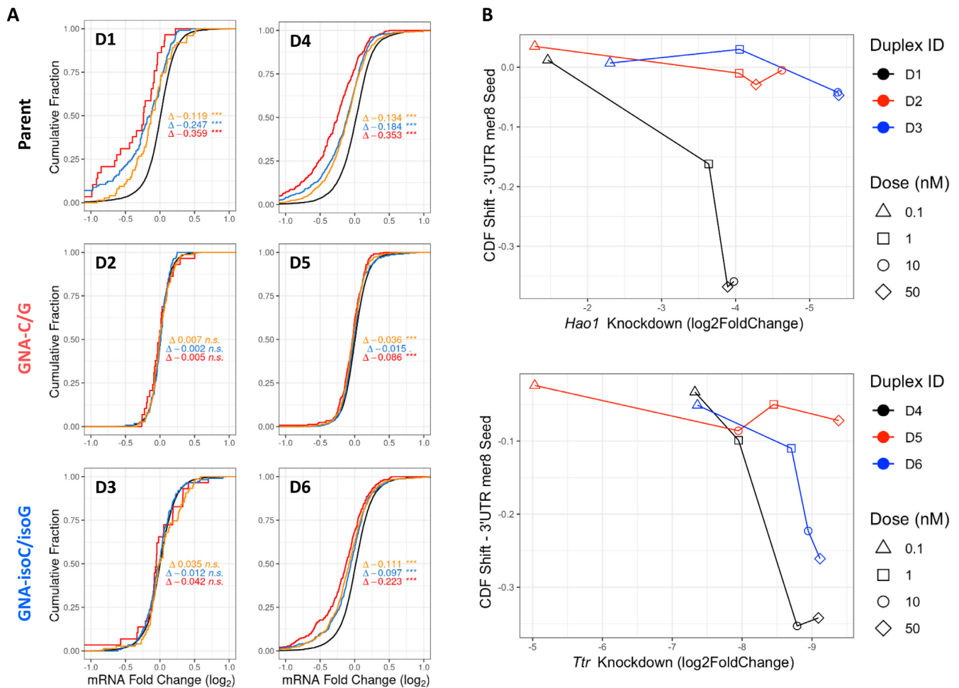
Figure 7. Evaluation of off- and on-target activity via RNA sequencing in primary mouse hepatocytes. (A) Cumulative distribution function (CDF) plots showing transcriptional dysregulation after transfection at a 10 nM dose of the indicated GalNAc-siRNAs. Each line represents the cumulative distribution of expression change among genes with or without the presence of the specified seed match in the 3'-UTR. The black line represents background genes lacking the specified seed matches below while the colored lines represent genes with at least one seed match, split by the identity of the strongest match (red = mer8, blue = mer7m8, yellow = mer7A1) (44). Delta values indicate the magnitude of each CDF shift versus background. (B) Plot of mer8 CDF shift versus on-target knockdown across various doses of the indicated GalNAc-siRNAs.
