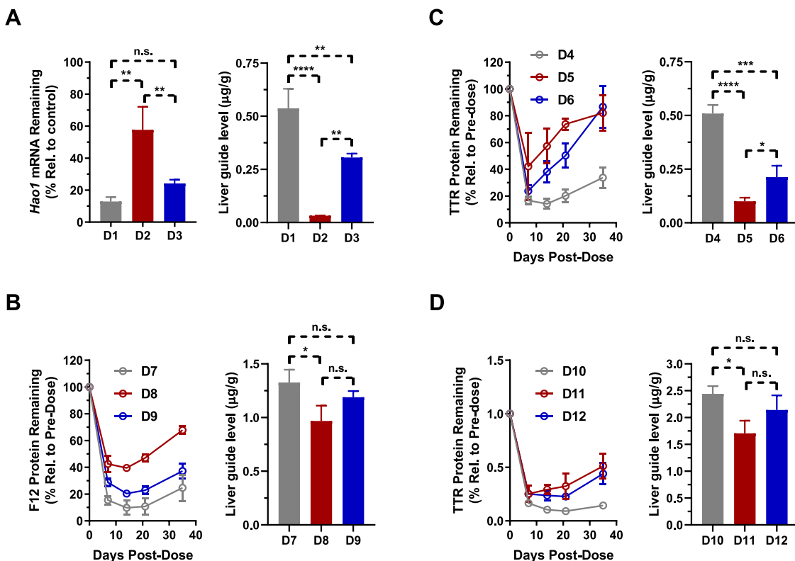
Figure 8. In vivo pharmacology (left of each panel) and guide liver levels (right of each panel) in mice after a single subcutaneous dose of parent or GNA-modified GalNAc-siRNAs. (A) Hao1 mRNA knockdown 7 days after a dose of 1 mg/kg of D1-D3 . (B) F12 protein knockdown after a dose of 1 mg/kg of D7-D9 . (C and D) TTR protein knockdown after a dose of 0.5 mg/kg ( D4-D6 ) or 1 mg/kg ( D10-D12 ) siRNA; * P < 0.05 , ** P < 0.01 , *** P < 0.001 , **** P < 0.0001 .
