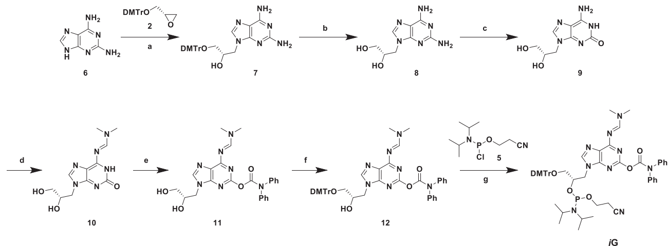
Scheme 2. Synthesis of ( S )-GNA-isoguanosine phosphoramidite iG . (a) NaH, DMF, 61%; (b) 80% aq. AcOH, 84%; (c) NaNO 2 , AcOH, H 2 O, 96%; (d) DMF-DMA, MeOH, 97%; (e) DPC-Cl, DIPEA, pyridine, 45%; (f) DMTr-Cl, pyridine, 55%; (g) DIPEA, MeIm, CH 2 Cl 2 , 80%. DMF-DMA = N,N -dimethylformamide dimethylacetal, DPC-Cl = diphenylcarbonyl chloride, DMTr-Cl = 4,4'-dimethoxytrityl chloride, MeIm = 1-methylimidazole.
