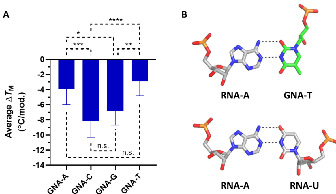
Figure 1. Reverse Watson–Crick base-pairing in GNA/RNA heteroduplexes. (A) Average change in T_M after incorporation of a single GNA nucleotide in positions 3–19 in a GalNAc-siRNA conjugate (21). (B) Example of RNA-A:( S )-GNA-T (top) and RNA-A:RNA-U (bottom) base pairs demonstrating a rotated GNA nucleobase orientation in a reverse Watson–Crick base pair. Adapted from the structure 5V1L in the Protein Data Bank (21); * P < 0.05 , ** P < 0.01 , *** P < 0.001 , **** P < 0.0001 .
