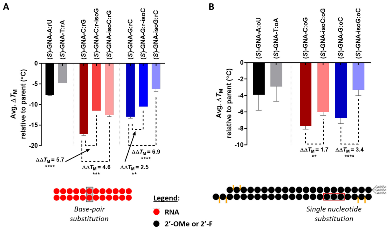
Figure 5. Impact of GNA nucleotide incorporation on duplex stability. (A) For the 12-mer RNA duplexes, the site of the modified base-pair is indicated by the black box (see Supplementary Table S1). Measurements were performed in 1× PBS at a duplex concentration of 2 \mu M and each data point is the average of two separate measurements relative to the unmodified parent. (B) The conjugate GalNAc-siRNA duplexes were modified with a single GNA nucleotide, and the site of incorporation is highlighted by the red box (g5, g6 or g7; see Supplementary Table S3). Measurements were performed on the fully modified GalNAc-siRNA duplexes (D1–D28) at a concentration of 1 \mu M in 0.1× PBS, and the data are represented as the average result across five different sequences relative to the parent GalNAc-siRNA not modified with GNA; * P < 0.05 , ** P < 0.01 , *** P < 0.001 , **** P < 0.0001 .
