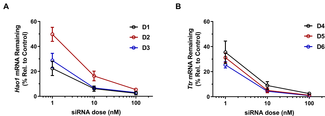
Figure 6. Free uptake silencing of parent and GNA-modified GalNAc-siRNAs (A) D1-D3 targeting the mRNA of Hao1 or (B) D4-D6 targeting the mRNA of Ttr in primary mouse hepatocytes.
