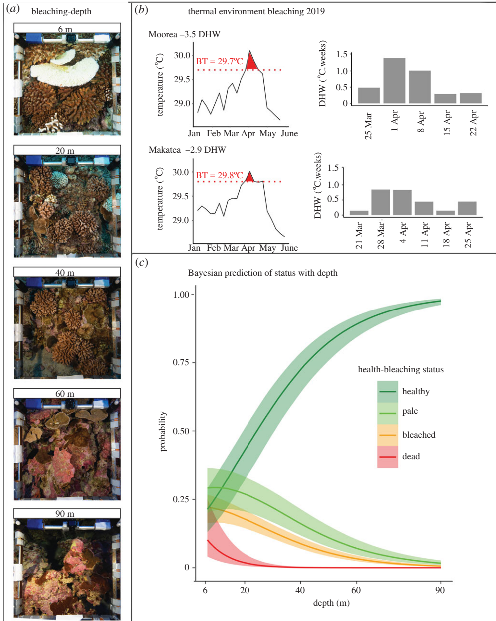
Figure 1. (a) Sample photo-quadrats at different depths. (b) Thermal environment with degree heating weeks (DHW) values using Satellite Coral Reef Watch Temperature. (Left) Sea surface temperatures during the bleaching episode. Red fill colour shows the exposure period above the bleaching threshold marked with a dotted line. (Right) Weekly development of the DHW. (c) Bayesian prediction probability of the likelihood of corals to be healthy, pale, bleached or dead as a function of depth.
