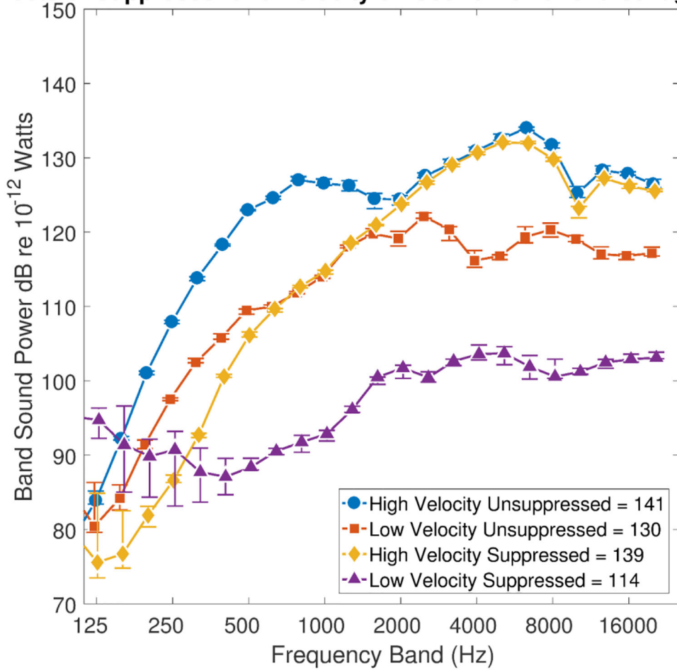
Figure 6. The sound power for each one-third octave frequency band, high-velocity/low-velocity ammunition, and for the suppressed/unsuppressed conditions for the .22 caliber Savage MK-11 rifle.
