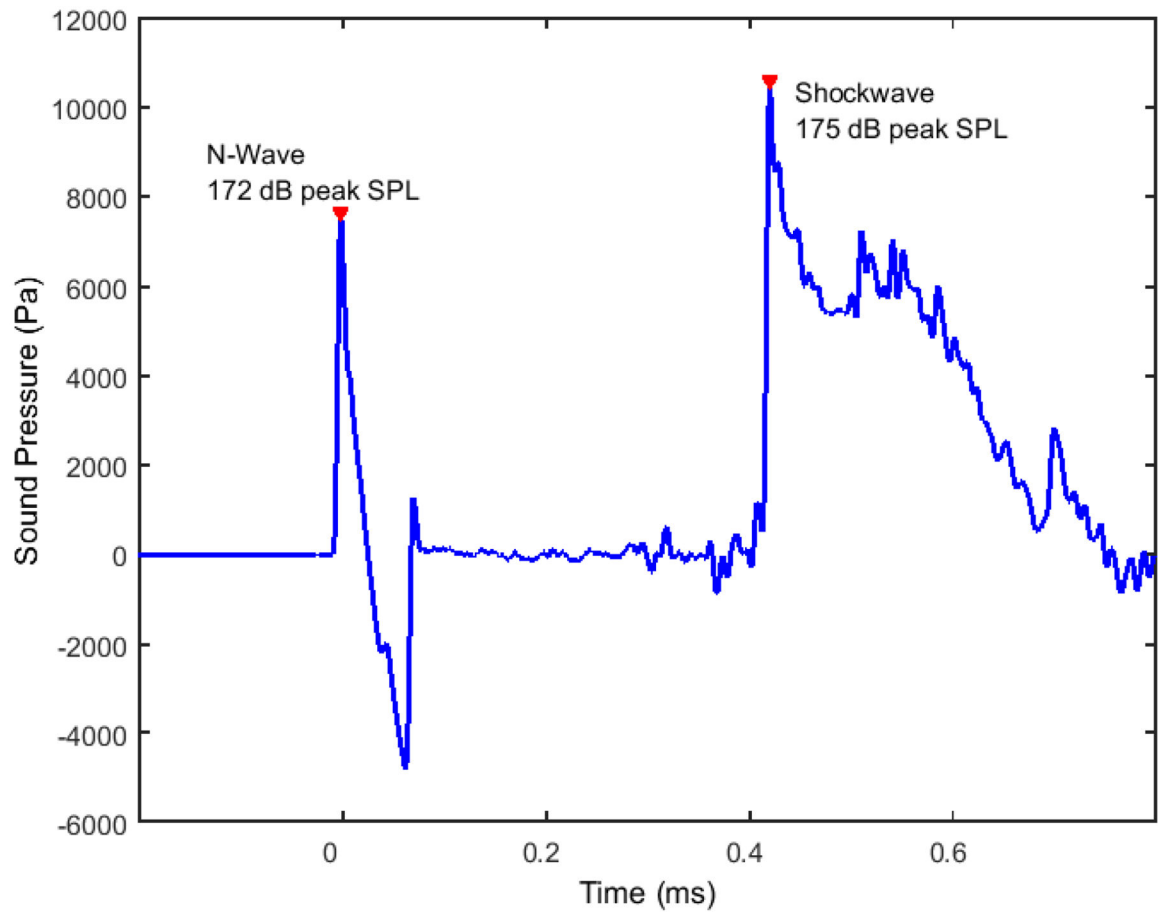
Figure 1. An example of an N-wave preceding the blast wave. The peak levels of the N-wave and shock wave are indicated with inverted triangles. Figure adapted from Rasmussen et al 2009, Figure 9.
