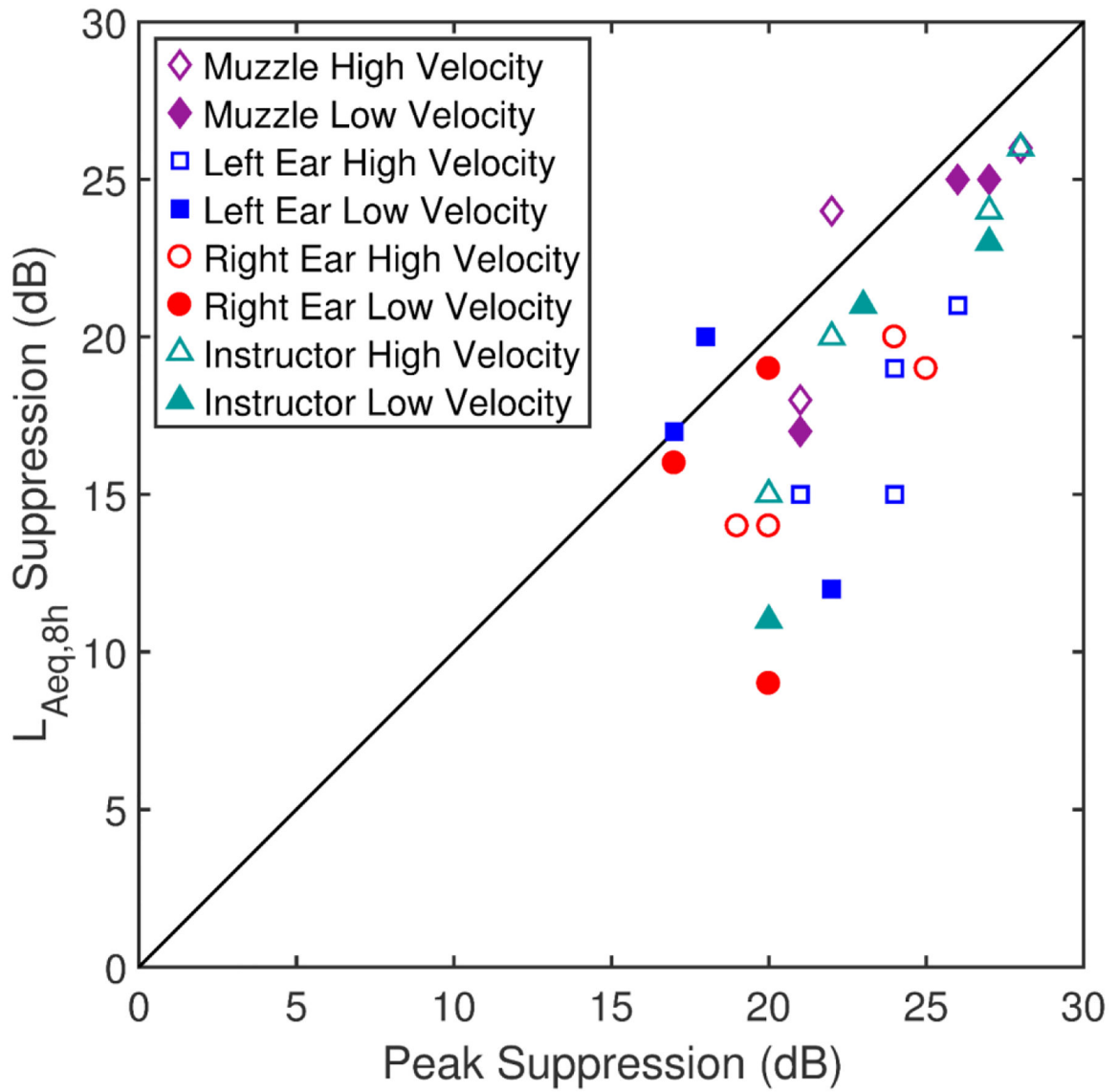
Figure 2. Comparison of suppressors' noise reduction assessed with change in peak level versus change of 8-hour A-weighted equivalent energy, L_{Aeq,8h} . Open symbols denote the high-velocity rounds and closed symbols are low-velocity rounds. The purple diamonds, blue squares, red circles, and cyan triangles are the reductions measured at the muzzle, left ear, right ear and instructor positions.
