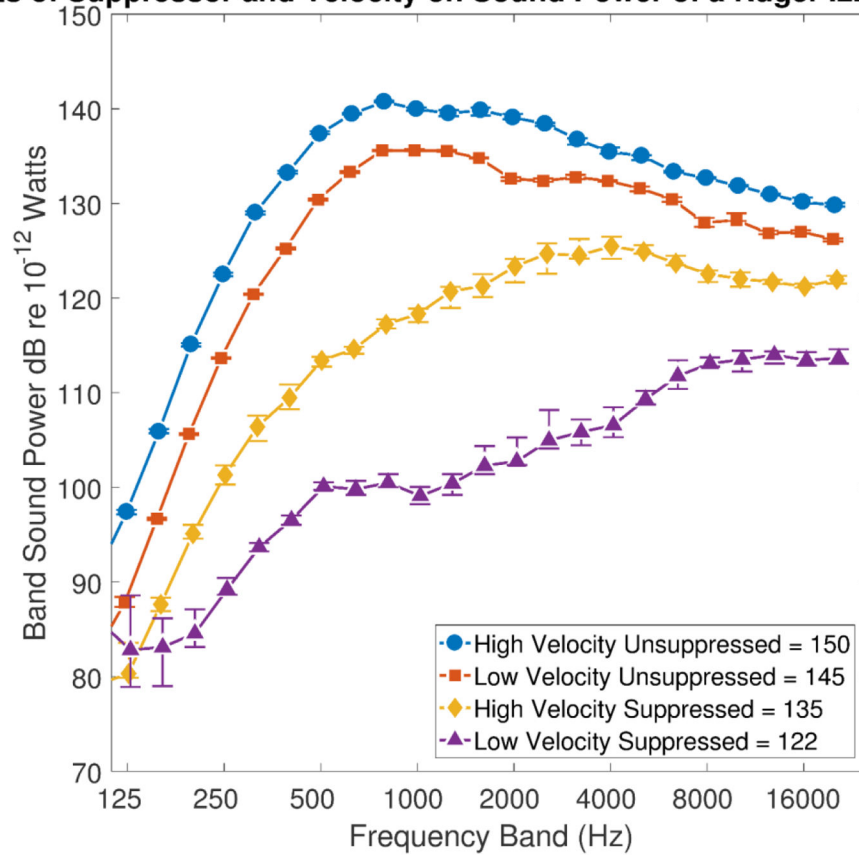
Figure 4. The sound power levels of the Ruger pistol at each one-third octave frequency band, high-velocity/low-velocity ammunition, and for the suppressed/unsuppressed conditions.
