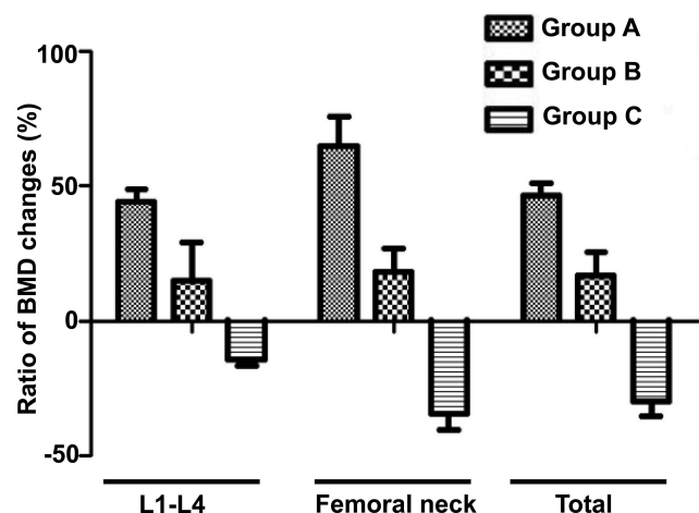
Figure 1 Observed BMD changes of HO patients after different treatments. BMD of L1–L4, the femoral neck and the total hip significantly increased (P < 0.01) after continuous treatment with a neutral phosphate solution (group A). There was no significant improvement in the BMD after intermittent treatment with a neutral phosphate solution (group B, P > 0.05). Patients not treated with a neutral phosphate solution showed decreased BMD (group C, P < 0.05).
