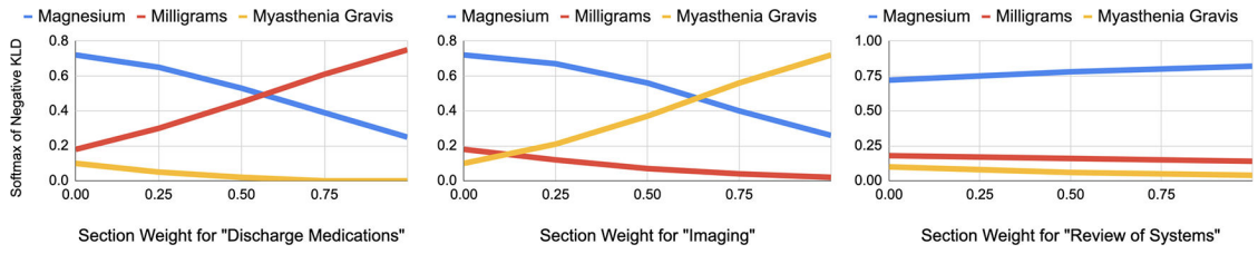
Figure 4: The latent sense distribution changes when manually interpolating the variational network weight between the word “MG” & different section headers.
