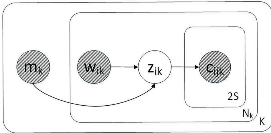
Figure 2: LMC Plate Notation.
