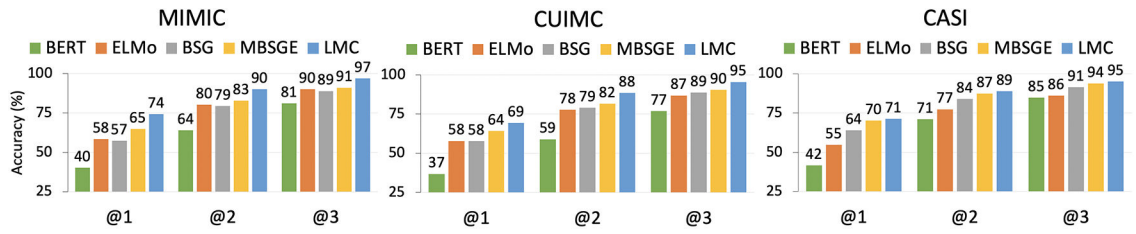
Figure 3: Average accuracy @K across 5 pre-training runs.
