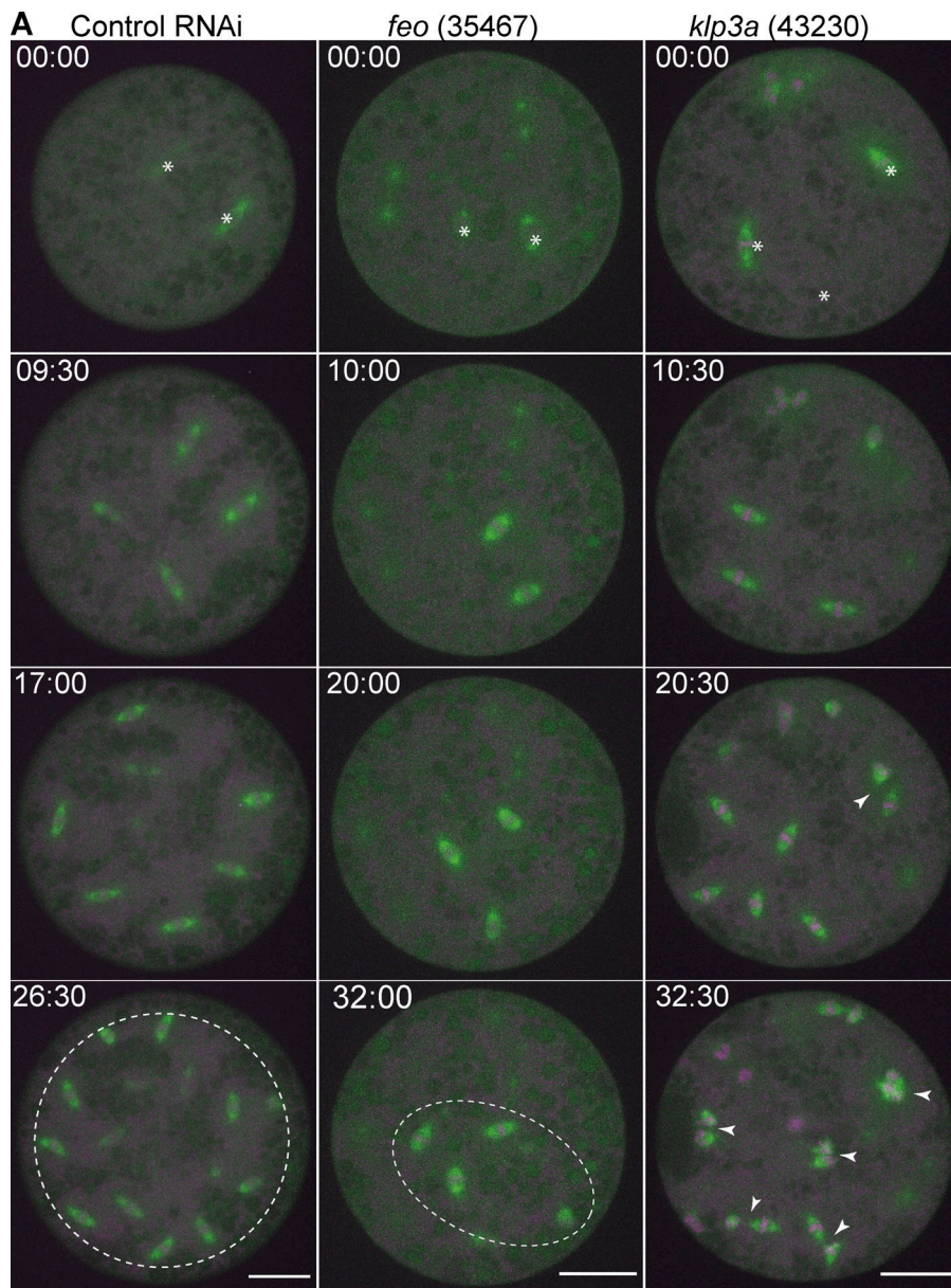
Figure 3. Knockdown of feo , klp3a , or klp61f by RNAi leads to defective nuclear distribution in preblastoderm embryo explants.
