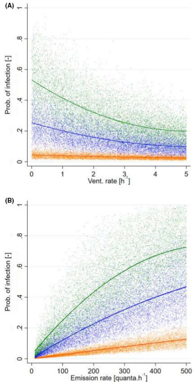
FIGURE 4 (A) Probability of infection simulated in a 150 \text{ m}^3 room for various loss rate due to ventilation ( \lambda_v ) and event duration: orange: 0.5 h, blue 1.5 h, green 3 h ( n = 30\,000 ). (4B) Probability of infection simulated in a 150 \text{ m}^3 room for various emission rates E and event duration: orange: 0.5 h, blue 1.5 h, green 3 h ( n = 30\,000 )
