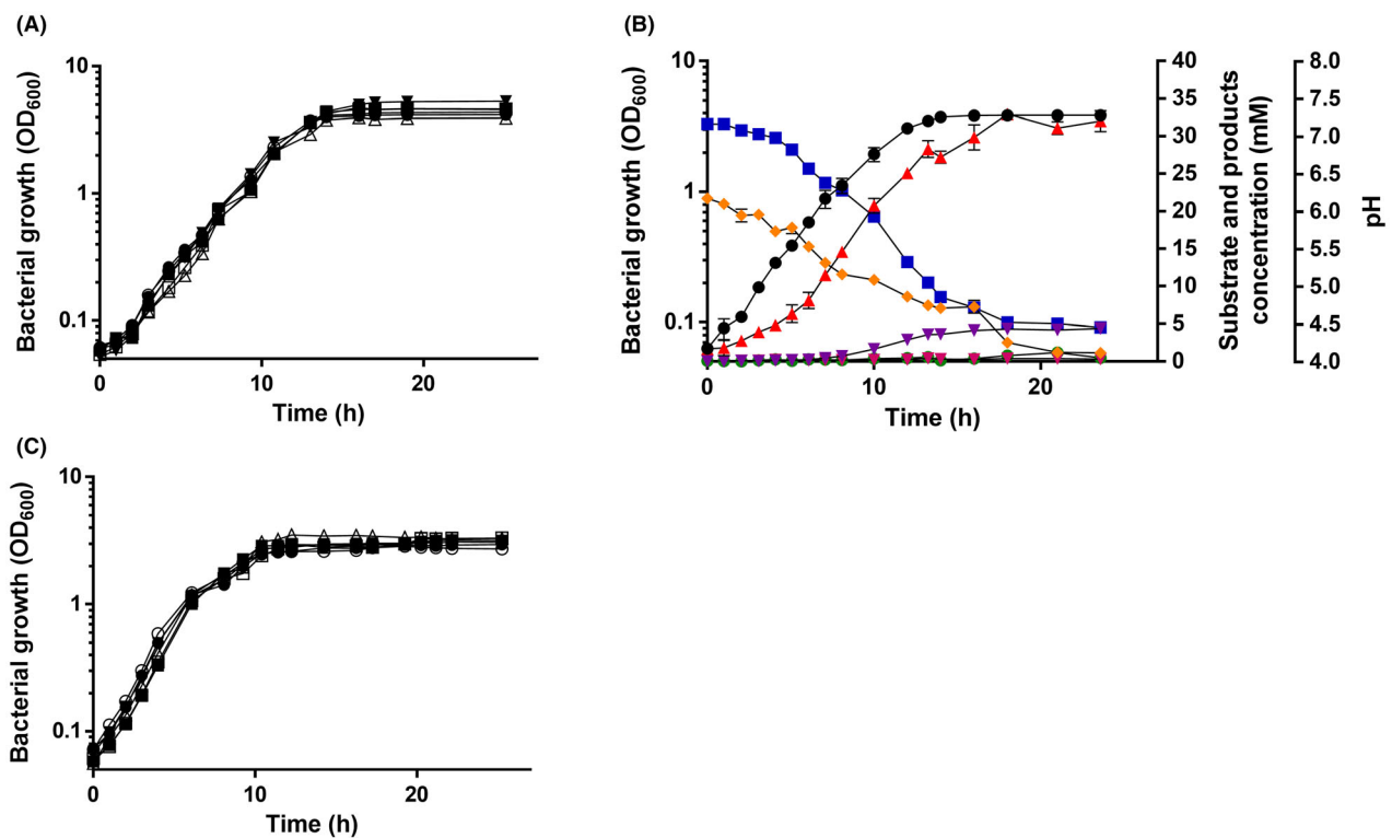
Fig. 2. Growth of E. limosum on glucose and fructose. E. limosum KIST612 was grown at 37^\circ\text{C} in 500 ml of carbonate-buffered basal medium (CBBM) (Chang et al. , 1999) with glucose under a \text{N}_2/\text{CO}_2 (80/20% [v/v]) atmosphere. Growth was followed by measuring the optical density (OD) at 600 nm.
