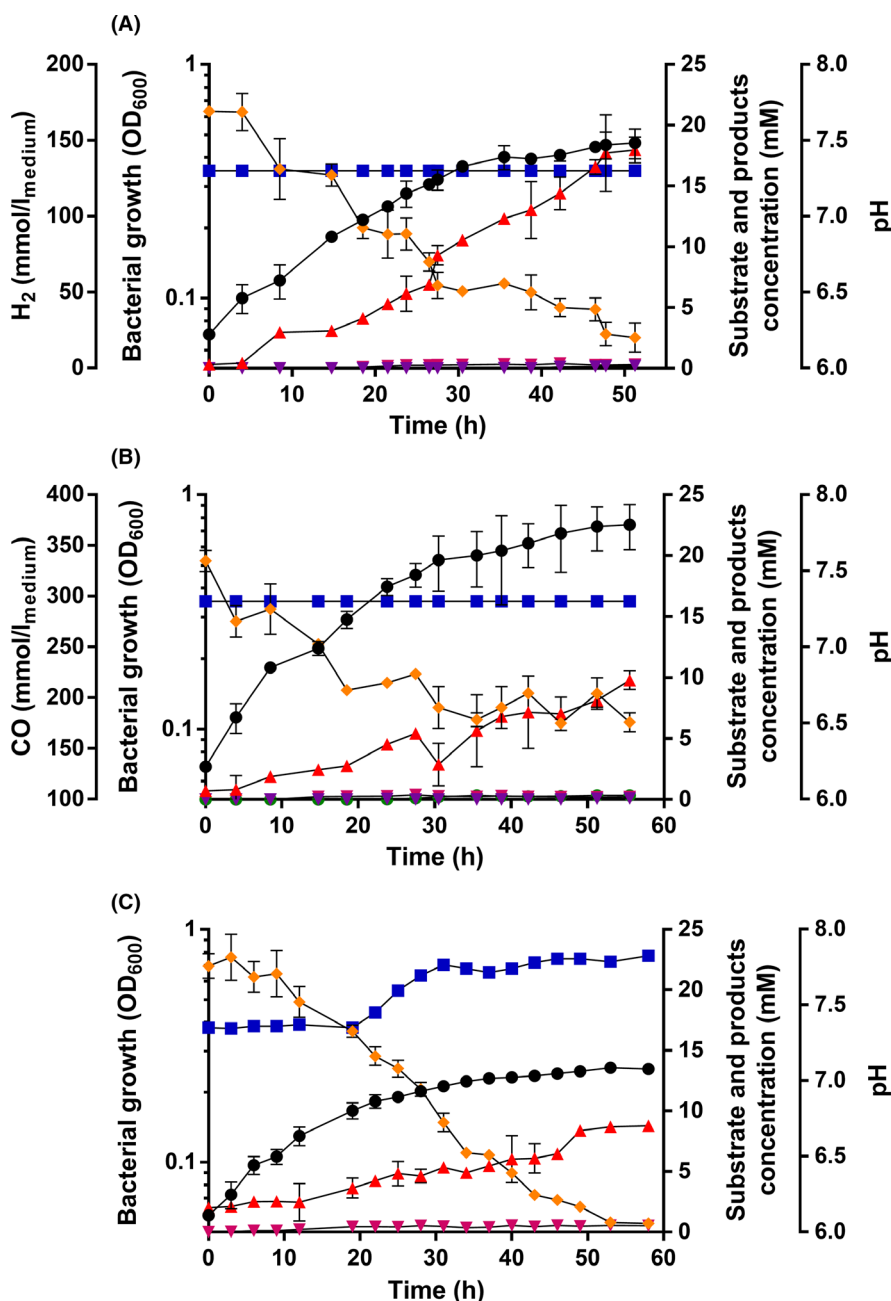
Fig. 3. Growth of E. limosum on H 2 + CO 2 , CO or formate.
