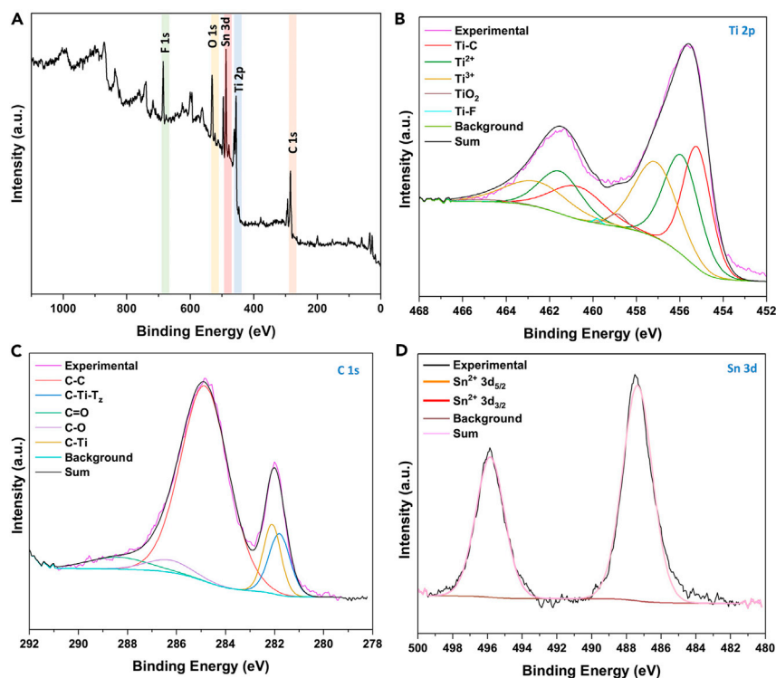
Figure 5. Deconvoluted XPS spectra of \text{Ti}_3\text{C}_2\text{T}_z nanosheets
