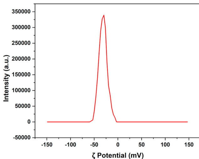
Figure 3. \zeta potential of delaminated \text{Ti}_3\text{C}_2\text{T}_2 nanosheets indicating the colloidal stability of aqueous dispersion of nanosheets
