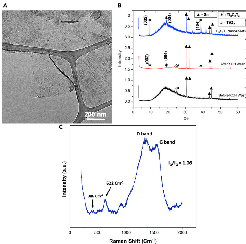
Figure 6. Characterization of \text{Ti}_3\text{C}_2\text{T}_z nanosheets
