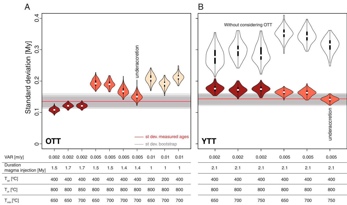
Fig. 4. Summary of the thermal modeling results for zircon crystallization. (A–B) The red line is the SD (st. dev.) of zircon ages for the natural OTT and YTT samples. The gray lines are SDs for the bootstrapped zircon age distributions. The violin plots present the distributions of SDs for 1,000 samples from a larger population, for the same number of measurements collected for the OTT ( n = 134 ) and the YTT ( n = 109 ). The colors of the violins relate to the VAR used in the model. The white violin plots show the results obtained without considering the removal of zircons by the OTT eruption. Each of the violin plots shows the results of models performed for different scenarios, as specified at the bottom of the figure. The best-fit models are considered those for which the violin plot overlaps with the gray lines.
