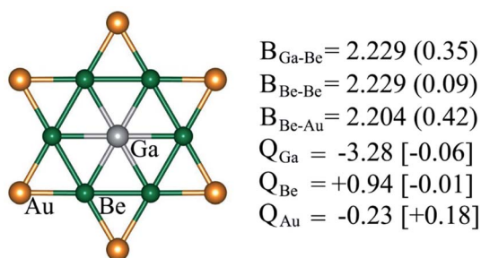
Fig. 3 Bond properties ( B , bond distances ( \text{\AA} ), WBIs (in parentheses)), NPA and Hirshfeld (in square brackets) charges ( Q , in |e| ) of \text{GaBe}_6\text{Au}_6^+ computed at the PBE0/def2-TZVP level.
