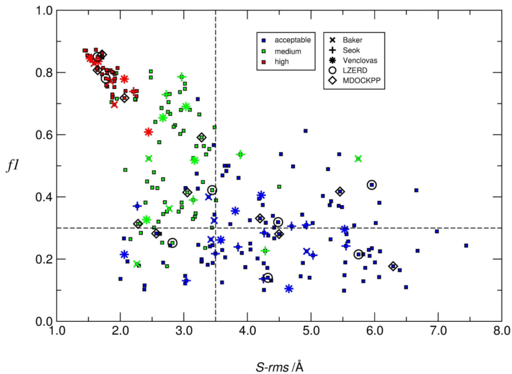
Figure 7: fI as a function of S-rms .
