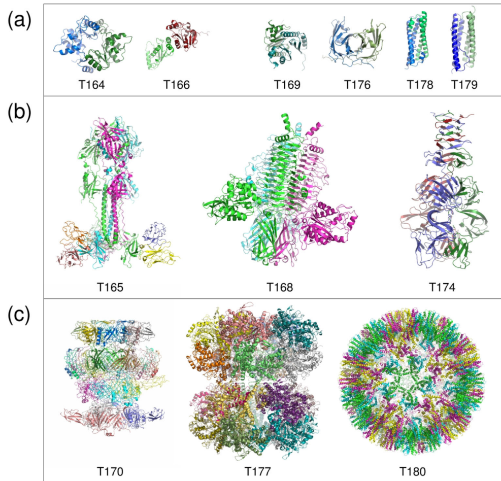
Figure 1: The Targets of Round 50.
