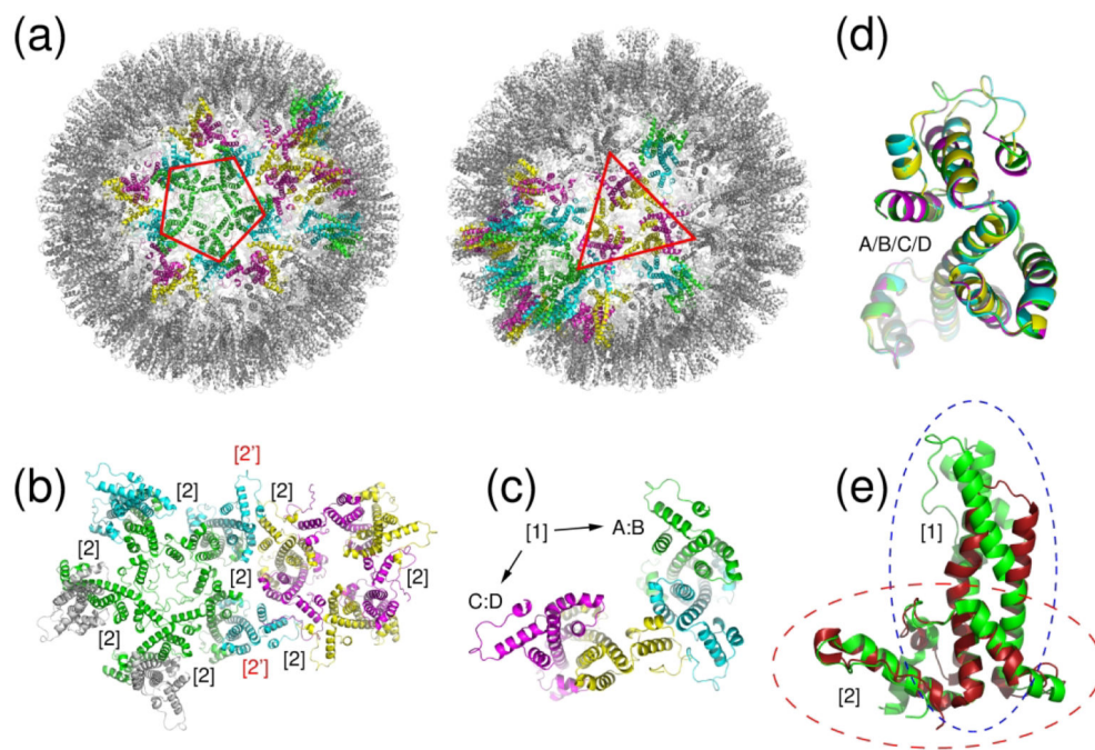
Figure 4: Subunit interactions and quasi symmetry of the duck hepatitis B virus capsid (T180/T1099)
