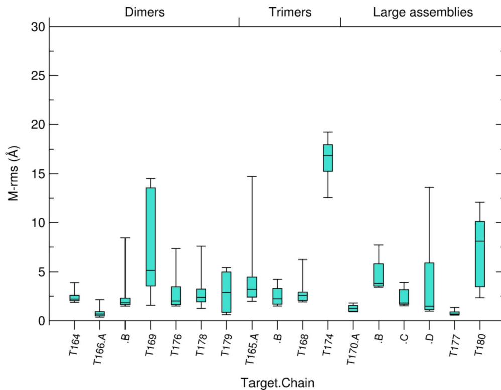
Figure 9: Model quality of individual protein subunits in assembly models of the 12 targets of Round 50.
