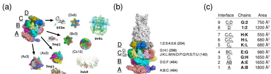
Figure 3: Subunit arrangement and interfaces of the T5 phage tail distal complex (T170/H1060).
