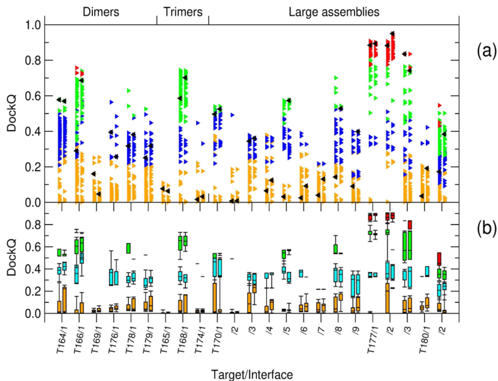
Figure 6: Global overview of the prediction performance for targets of Round 50. Shown are the distributions of the DockQ values computed for the top-five models submitted by all predictor and scorer groups for individual targets of Round 50. (a) Scatter plots of DockQ values for individual models submitted by predictors (left column) and scorers (right column) for individual targets. The targets are labeled by their CAPRI target number and interface rank. Individual points are color-coded according to the CAPRI model quality category; yellow: incorrect; blue: acceptable; green: medium; red: high. For each target, a baseline-level prediction, represented by the best model of the top-performing automatic server (MDOCKPP; see Table 2), is represented by black triangles. (b) The same information presented as boxplot distributions (whiskers at 9 th and 91 st percentiles) of models submitted for each target and prediction category; color coding is as for the upper panel, but with a lighter shade of blue for better visibility.
