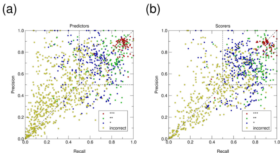
Figure 5: Global landscape of the interface prediction performance.
