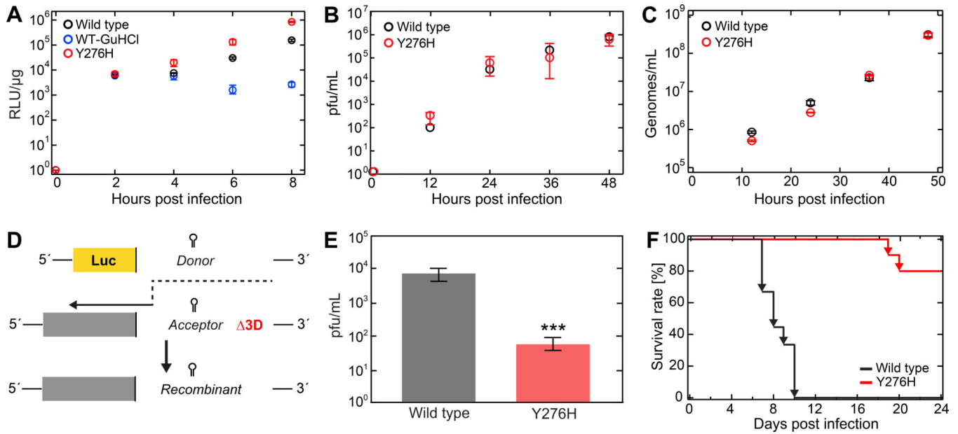
Figure 2. EV-A71 Y276H RdRp variant exhibits significance decrease in recombination efficiency and virulence.
