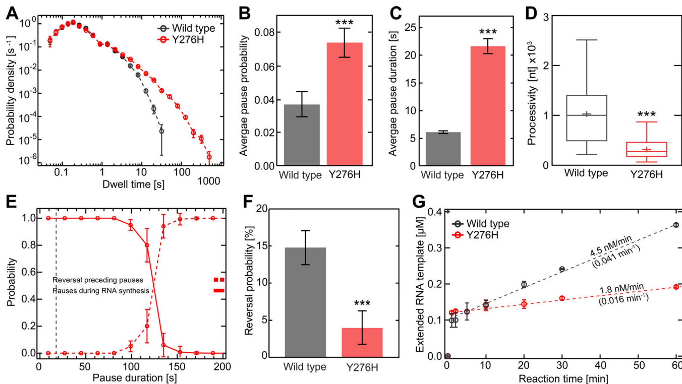
Figure 3. EV-A71 Y276H RdRp variant is impaired for copy-back RNA synthesis.
