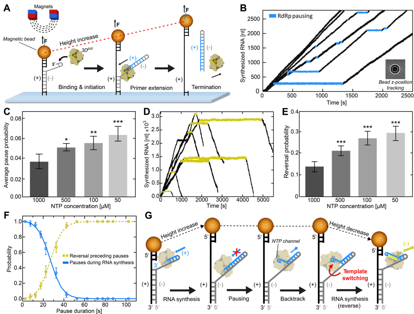
Figure 1. Magnetic tweezers assay of EV-A71 RdRp reveals pause-dependent copy-back RNA synthesis.
