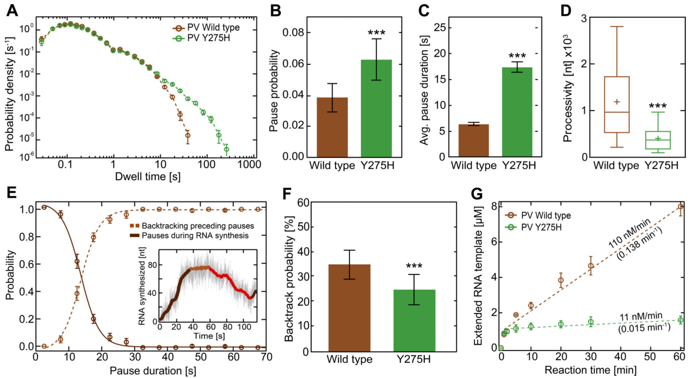
Figure 4. PV Y275H RdRp is impaired for backtracking. (A) Superimposed dwell-time distributions of poliovirus Y275H RdRp variant (green) and WT (brown) RdRp. The 275H variant exhibits a broad increase in the probability and duration of long pauses compared to WT. The dwell-time window was set to 4 nt, and the error bars (AVG \pm SD) result from bootstrapping with 1,000 iterations. (B-D) Quantification of the data in panel (A). In comparison to WT RdRp, the Y275H variant shows a significant increase in (B) average pausing probability ( \pm SD) and (C) average apparent pause duration ( \pm SEM) during RNA synthesis. The processivity (D) is significantly decreased for the Y265H RdRp variant compared to WT. (E) The probability of observing pauses of specified durations during PV WT RNA synthesis (dark brown) co-plotted with the probability of observing backtracking (light brown dashed line); the crossover point is found at \sim 14 s. (F) The Y275H variant (green) shows a significantly decreased backtracking probability (AVG \pm SD) than WT RdRp (brown). (G) In vitro bulk RNA synthesis assay results (AVG \pm SD; n = 3 repetitions) showing the amount of extended Sym/SubU template for PV WT and Y275H RdRp over time. Dashed lines represent linear regressions fitted to the data, revealing significantly lower approximated rates of RNA extension (values above the dashed lines) and turnover (values below the dashed lines; unit: RNA min -1 RdRp -1 ) for the Y275H RdRp variant compared to WT. Statistical analyses were performed using unpaired, two-tailed t-tests (significance level p: *** 0.001).
