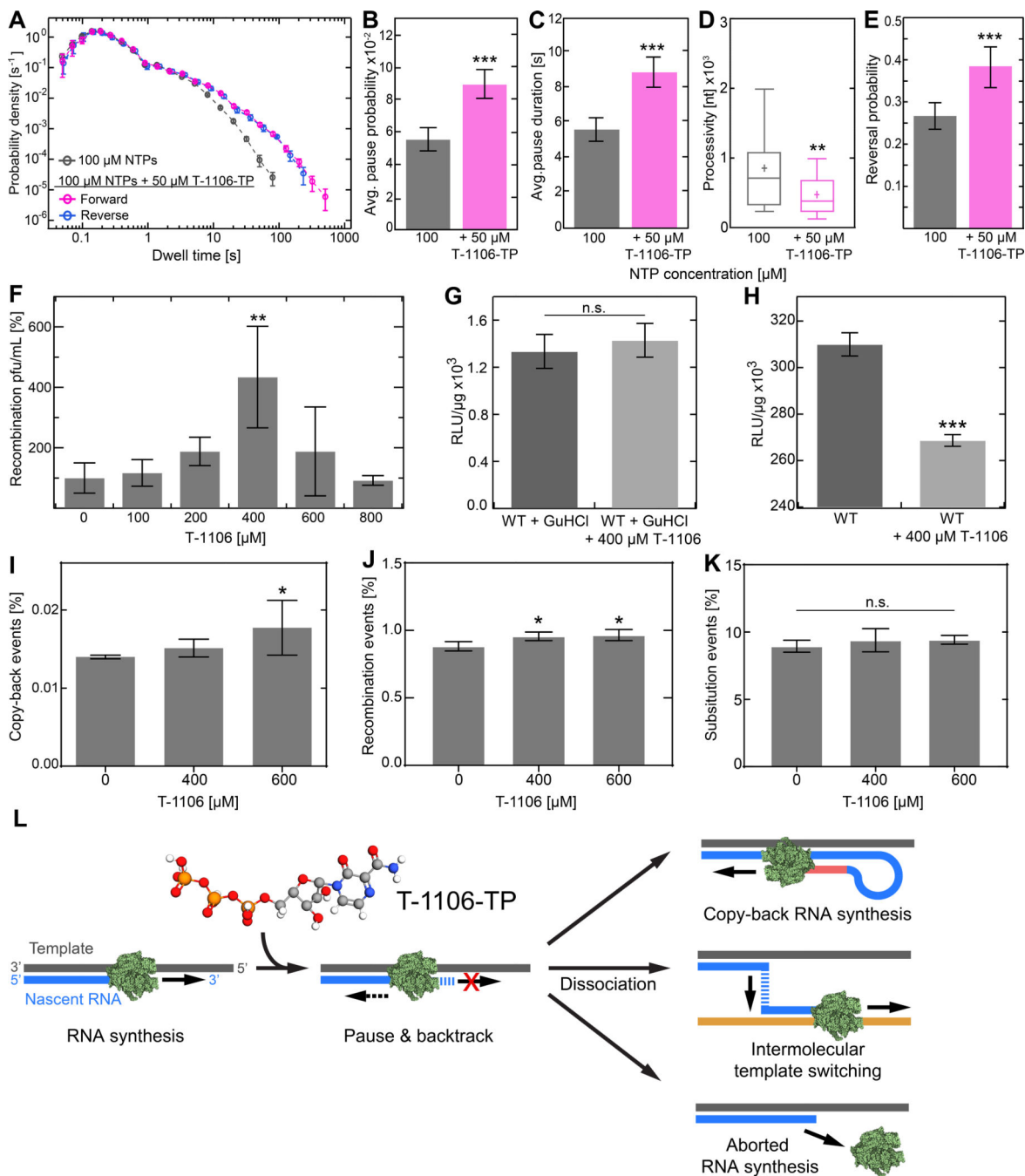
Figure 6. Pyrazine carboxamide T-1106 induces an increase in intra- and intermolecular template switching in vitro and in cell.
