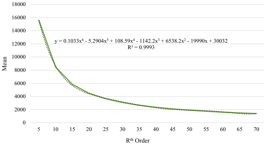
Fig. 3 Mean distribution of R th order extremes
