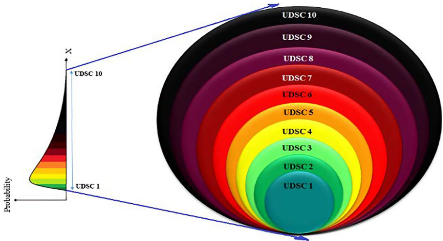
Fig. 2 Probability distribution and severity levels
