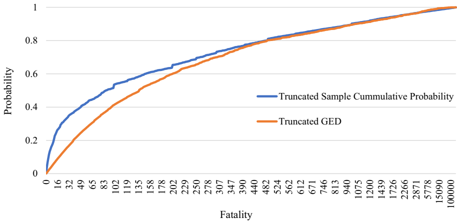
Fig. 4 Cumulative sample distribution of fatalities with an approximate 70 th order GED
