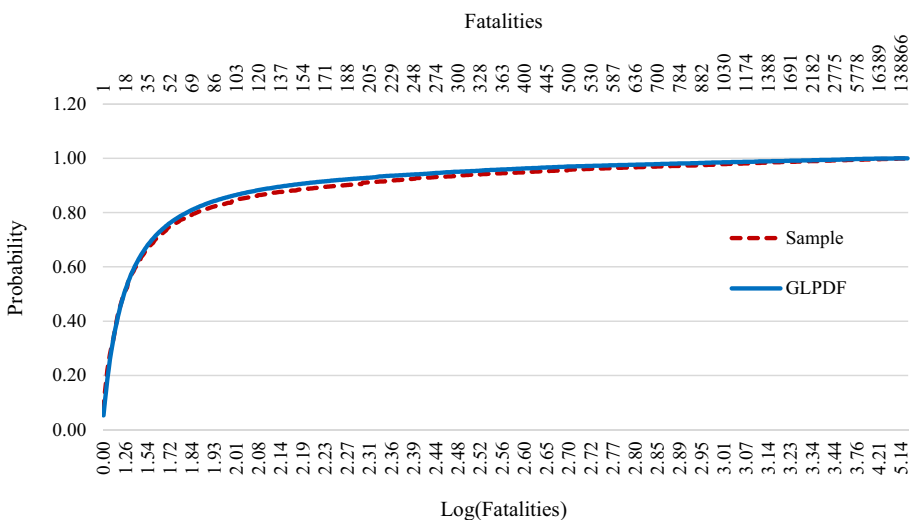
Fig. 1 Cumulative sample distribution of fatalities in a natural logarithm scale with an approximate GLPDF
