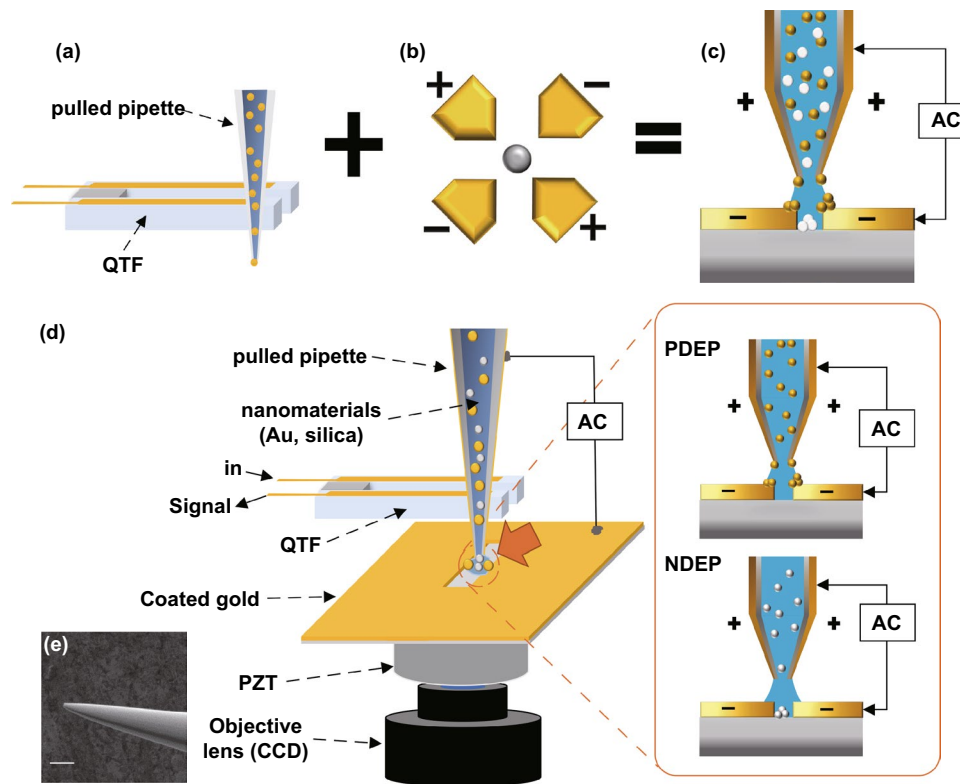
Fig. 1 Schematic diagram of the experiment. a QTF-AFM with a pulled pipette system. It has strength in efficient low-volume liquid delivery. b Quadrupole DEP trap. If the Clausius–Mossotti factor is below zero, solutes receive a negative-DEP force and go to the center of the electrodes. c We propose the DEP-based material-selective deposition technique using the pipette-AFM system. The pipette-AFM delivers the low-volume solution to the desired position and DEP forces deposited nanoparticles on the edge or middle position of electrodes. Yellow particles show the positive-DEP effect and white particles show the negative-DEP effect. d Detailed schematic diagram of the experimental setup. XY positioning of the pipette on the scratched gap is enacted while watching the optical microscope image of CCD in real-time, and the Z positioning (approach and retract) of the pipette is enacted under QTF-AFM feedback. An AC voltage is applied between the coated Au layer on the glass substrate and the surfaces of the Au-coated pulled pipette. e Detailed SEM image of the coated pulled pipette, 10 μm scale bar
