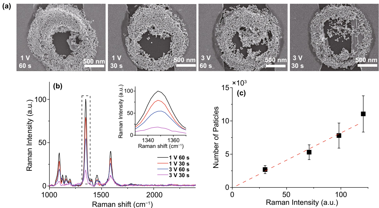
Fig. 4 SERS results of various PDEP Au nano-aggregates samples. a SEM images of Au nano-aggregates deposited by PDEP; 500 nm scale bar. b SERS spectra of various Au nano-aggregates coated with 4-nitrobenzenethiol; the inset graph is the expanded spectra in the dotted line (nitro group). c Raman intensity and particle count graph. The ratio of Raman intensity of peaks in the inset graph of b is linearly well-fitted (red dashed line) with the ratio of the number of Au nanoparticles, which indicates that Au nanoparticles enhanced Raman signal. Therefore, the system can be used for the fabrication of the nano-micro SERS platform by the enrichment of nanoparticles such as in the coffee-ring effect
