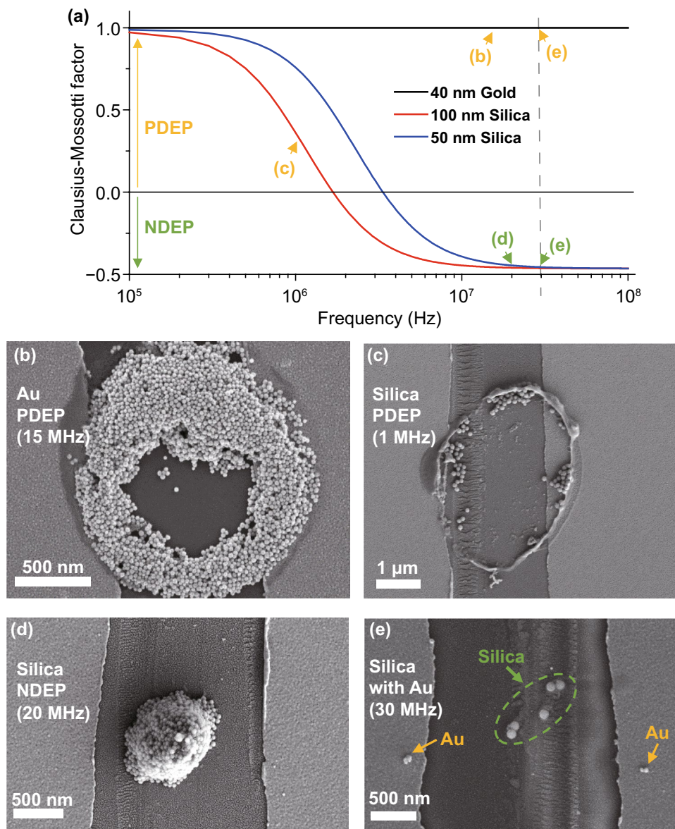
Fig. 3 SEM images of PDEP and NDEP experiments. a Clausius–Mossotti factor ( f_{CM} ) of nanoparticles used for experiments. Several characteristics ( \epsilon_{m/p} , \sigma_{m/p} , \sigma_{bulk} , K_s ) of Au and silica nanoparticles are from reference [29]. The X-axis is a log scale of the frequency (Hz). Signs of f_{CM} change at \sim 2 MHz (100 nm silica), \sim 4 MHz (50 nm silica), and f_{CM} of 40 nm Au always has a plus sign in the 0.1–100 MHz range. Arrows show the frequencies used, and colors indicate PDEP (yellow) or NDEP (green). b PDEP result of Au nanoparticles with 40 nm diameter Au nanoparticles, \sim 2 \mu m diameter pipette with R_{inner}/R_{outer} ratio = 0.7, V_{peak} = 1.0 V, and 15 MHz frequency. Particles are attracted to surface electrodes of the substrate and the pipette. c PDEP result of silica nanoparticles with 100 nm diameter silica nanoparticles, \sim 2 \mu m diameter pipette, V_{peak} = 2.5 V and 1 MHz frequency. Particles show the same tendency as in a . The concentration and surfactants of nanoparticle solutions result in differences between b and c . d NDEP result of silica nanoparticles with 50 nm diameter silica nanoparticles, \sim 1.5 \mu m diameter pipette, V_{peak} = 2.5 V, and 20 MHz frequency. Particles move off to the surface electrodes of the substrate and pipette and gather around the center of the pipette. e Sorting result of the mixed solution with 100 nm diameter silica nanoparticles and 20 nm diameter Au nanoparticles, V_{peak} = 2.5 V, and 30 MHz frequency. Silica nanoparticles in the green circle show NDEP and Au nanoparticles next to the yellow arrows show PDEP
