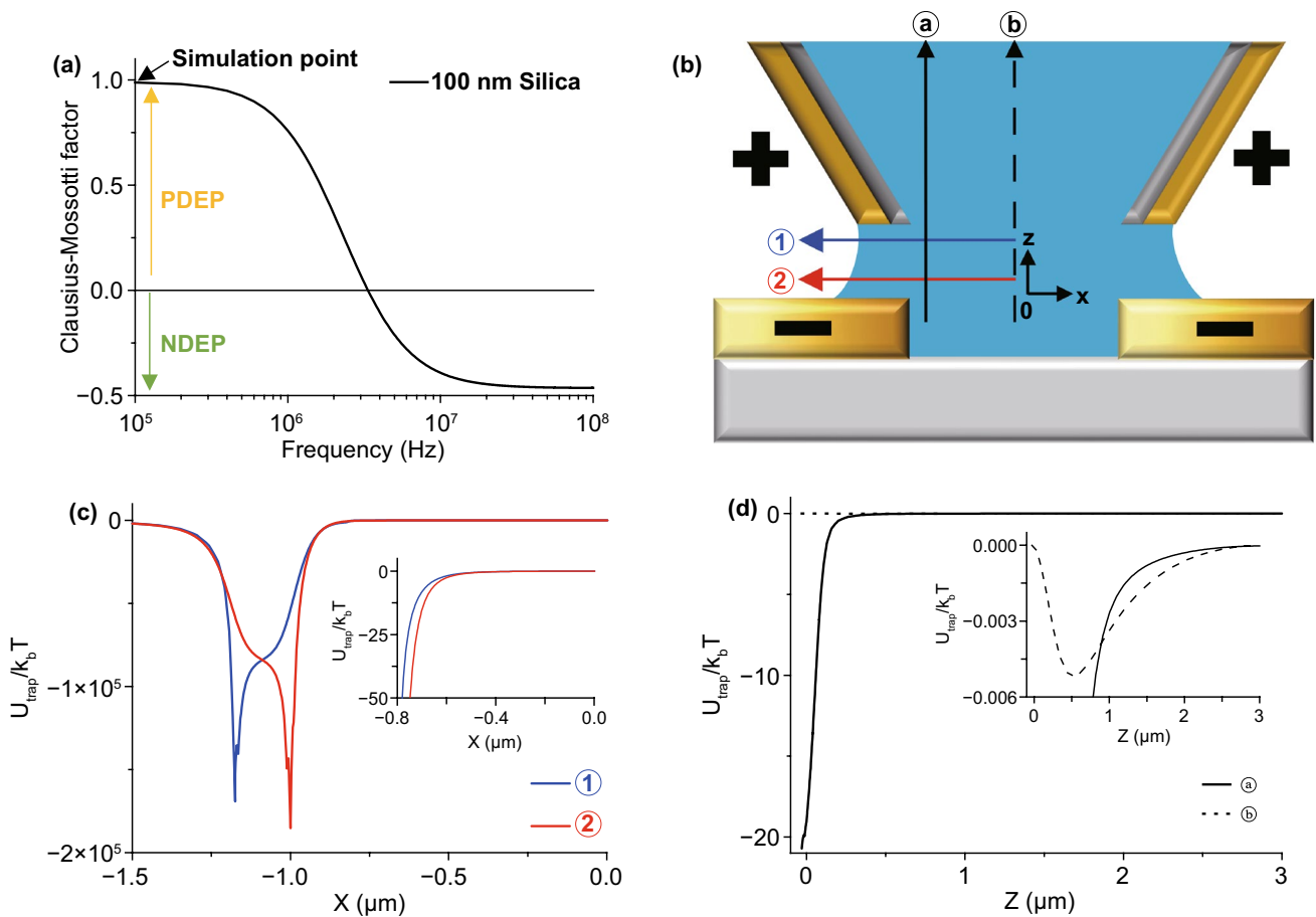
Fig. 2 a An example graph of Clausius–Mossotti factor ( f_{CM} ) of 100 nm diameter silica nanoparticles. The sign of f_{CM} determines PDEP or NDEP. The critical frequency of the sign is almost 3 MHz in this case. b Schematic diagram of the experiment with arrows for the X- and Z-directions. The phase of electrodes is determined by the simulation in Fig. S1. c Simulation graph of PDEP ( f_{CM} = 1.0 ) trap energy vs. Brownian motion along the X-axis. V_{peak} = 1.0 V, 15 MHz frequency of AC voltage, 100 nm diameter of the particle, 2.0 μm gap size, and 2.35 μm outer diameter of the pipette with a 0.7 R_{inner}/R_{outer} ratio. The trap energy rapidly increases around the edge of electrodes near the outer diameter of the pipette at \textcircled{a} ( \pm 1.175 μm) and substrate at \textcircled{b} ( \pm 1.0 μm), so the particles affected by the PDEP force are supposed to move to the edge of the electrodes. The inset image shows an expanded graph near the center; it shows the same direction for the PDEP force. The NDEP case shown in Fig. S3 and the particles affected by NDEP gather around the center near zero. d Simulation graph of the DEP trap energy vs. Brownian motion along the Z-axis with the same conditions as c . The particles affected by PDEP force are supposed to move downward at \textcircled{a} but the particles affected by NDEP go upward. However, in the inset graph, the Brownian motion energy is much bigger than the z-direction DEP trap energy at \textcircled{b} , so particles are not affected by the DEP force in the Z-direction except near \textcircled{a}
