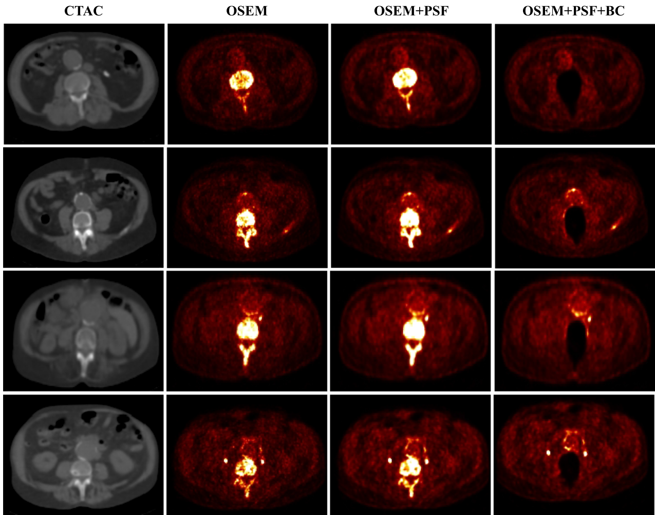
Figure 1. CT images and PET reconstructed images of four indicative patient datasets, showing a high ^{18}\text{F} -NaF uptake in the bone and the aneurysm. The activity contribution from the bone was removed in OSEM + PSF + BC.
