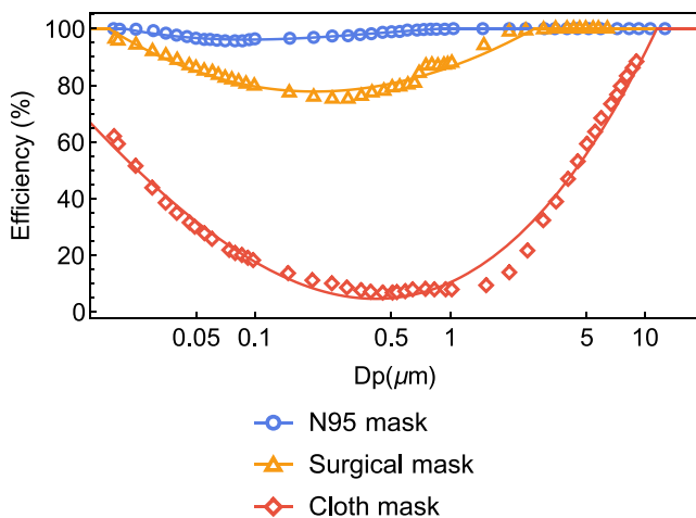
FIGURE 6 The filtration efficiency of N95 mask, surgical mask, and cloth mask for particles with diameter ranged from 0 to 20 \mu\text{m}
