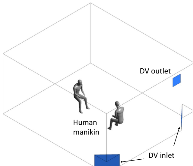
FIGURE 5 Geometry model of the environmental chamber for computational fluid dynamics simulation
