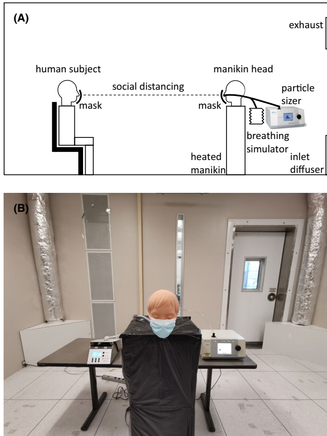
FIGURE 1 (A) Illustration of measuring size distribution of inhaled droplets when wearing face masks in various social distancing in the environmental chamber. (B) Photograph of the measurement devices in the environmental chamber
