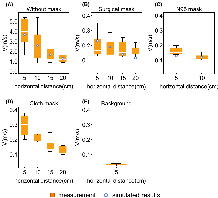
FIGURE 10 Measured and simulated respiratory air velocity along the horizontal distances when coughing (A) without face mask; (B) with surgical mask; (C) with N95 mask; and (D) with cloth mask as well as (E) background air velocity without respiratory activity
