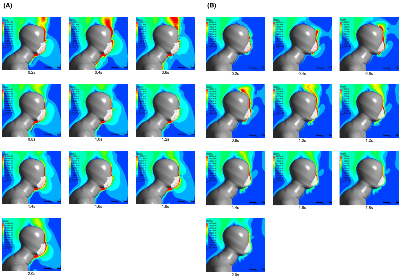
FIGURE 11 Computational fluid dynamics simulated air velocity distribution within 2 s when infected “patient” coughing while wearing (a) surgical mask and (b) N95 mask
