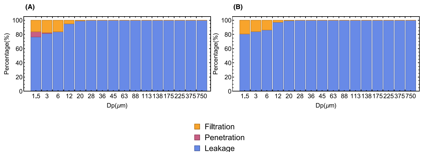
FIGURE 13 The percentage of exhaled particle filtered by face mask, penetrating the mask and moving through the leakage by computational fluid dynamics simulation for (A) surgical mask and (B) N95 mask
