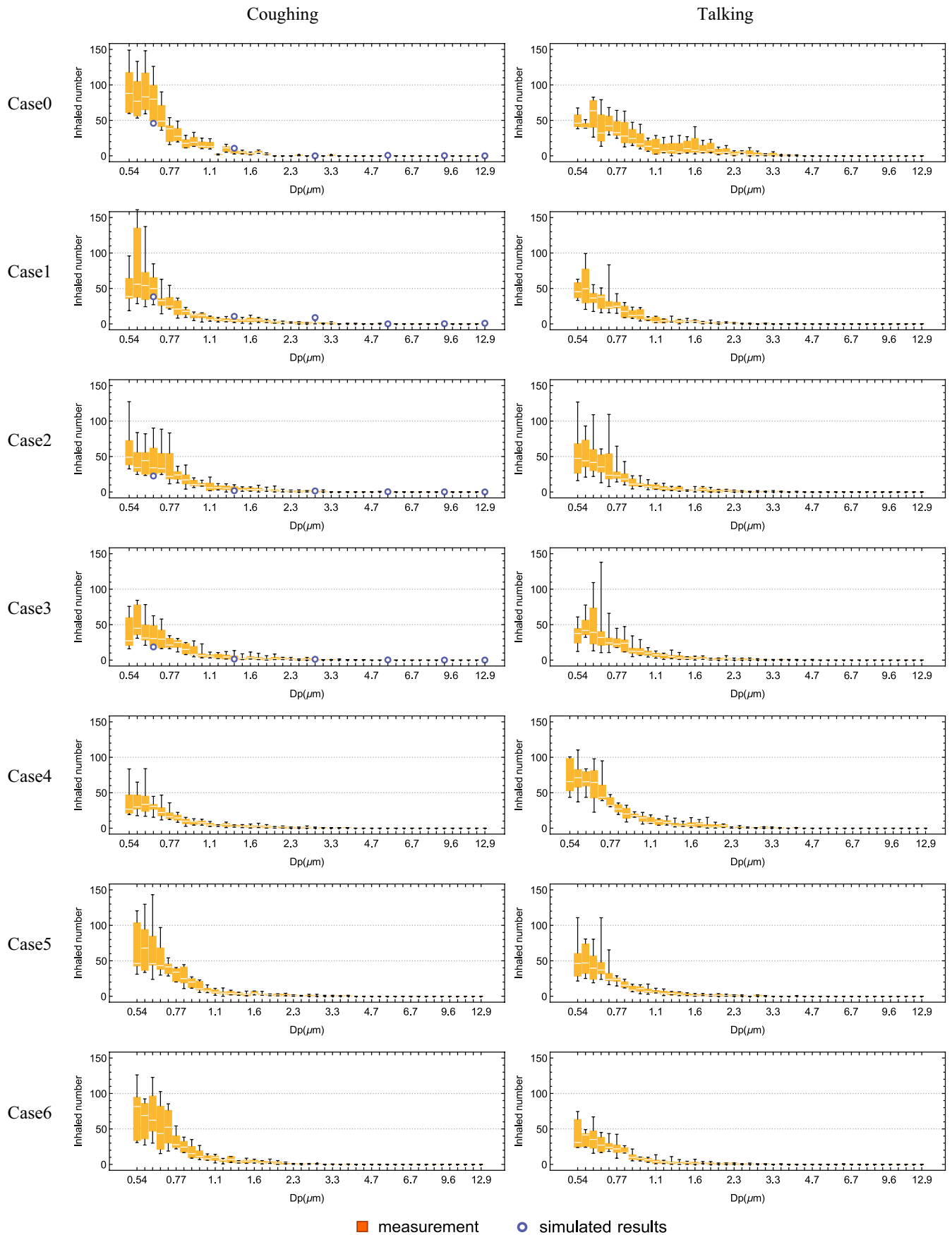
FIGURE 8 Measured and simulated size distribution of particles inhaled by the susceptible occupant that accumulated in 1 minute after the infected “patient” coughing/talking for the cases listed in Table 1
