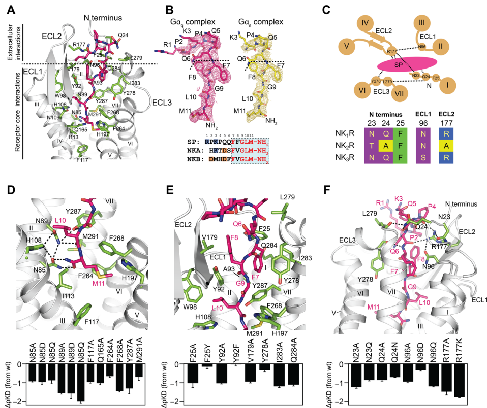
Fig. 2. Interactions of the endogenous agonist SP with NK 1 R. (A) SP (stick representation, carbons depicted in pink) establishes a host of interactions with the receptor transmembrane core and the extracellular receptor surface (receptor-interacting residues depicted as sticks with green carbons). (B) Processed cryo-EM maps of SP in the NK 1 R:G q complex (colored in pink) and the NK 1 R:G s complex (colored in yellow) contoured at 4.5 \sigma . Bottom: The amino acid sequences (numbers on top correspond to position in SP) of the three neuropeptides SP, NKA, and NKB are indicated by residues of the conserved ligand C terminus highlighted in red, and the C-terminal amide is shown. Negatively and positively charged residues are highlighted in orange and blue, respectively. (C) Schematic representation of the polar network shaping the extracellular receptor surface for SP binding, indicating the hydrogen bonds detected in the structure. Bottom: Alignment of residues involved in specific side-chain interactions of the polar network are shown, comparing NK 1 R with NK 2 R and NK 3 R. Framework residues of ECL3 only interact via backbone hydrogen bonding and are therefore not included in the alignment. (D to F) Close-up on the interactions of the amidated SP C terminus at the bottom of the orthosteric binding pocket (D), the interactions of the neurokinin-conserved C-terminal portion of SP with the hydrophobic interaction surface of helices VI and VII of NK 1 R (E), and the polar network at the extracellular receptor surface (F). Bottom: Agonist affinity profiles of selected mutants compared to wild-type NK 1 R are shown. pK D values were derived from whole-cell saturation binding experiments (table S1). Data are shown as means \pm SEM from three to six independent experiments performed in duplicate.
