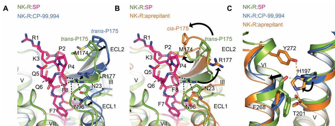
Fig. 5. The insurmountable antagonist-bound NK 1 R state prohibits SP binding. (A) Superposition of agonist-bound NK 1 R:SP:G q (green) with the surmountable antagonist CP-99,994-bound NK 1 R (PDB ID: 6HLL) (blue) reveals a slightly outward-moved but similar ECL2 conformation for the antagonist conformation. Note the small movement of R177 ECL2 . (B) Superposition of agonist-bound NK 1 R:SP:G q with the insurmountable antagonist aprepitant-bound NK 1 R (PDB ID: 6HLO) reveals an inward shifted and twisted ECL2 in the insurmountable conformation that clashes at M174 ECL2 with P 4 of the endogenous agonist and also poses R177 ECL2 away from its central position in the polar network at the extracellular receptor surface. (C) Superposition of agonist-bound NK 1 R:SP:G q , CP-99,994- and aprepitant-bound NK 1 R showing the hydrogen bonds (indicated as orange, dotted lines) that lock helices V and VI in the insurmountable conformation. The rotamer orientation of H197 5.39 in the insurmountable conformation prevents the necessary inward movement of helix VI and the formation of a new hydrogen bond between H197 5.39 with the backbone carbonyl oxygen of F268 6.55 (indicated as green, dotted line) in the active state.
