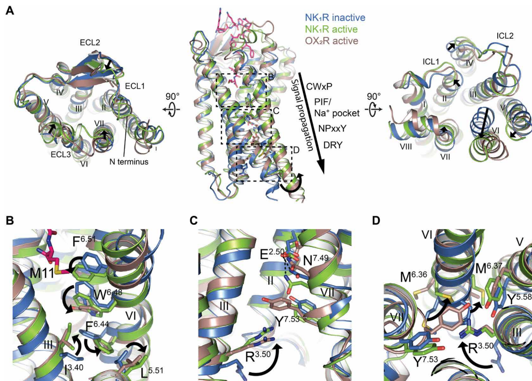
Fig. 3. Molecular characteristics of NK 1 R activation by SP. (A) Superposition of the active-state NK 1 R:SP:G q (green) with the inactive-state crystal structure of NK 1 R in complex with the antagonist CP-99,994 (PDB ID: 6HLL) (blue) and the active-state OX 2 R:G q complex (PDB ID: 7L1U) (brown). Relative changes from inactive to active NK 1 R are indicated by black arrows. Left: extracellular view, right: intracellular view, middle: side view with approximate position of conserved motifs involved in receptor activation indicated, and sections of the close-up views in (B) to (D) highlighted by dotted boxes. (B to D) Close-up views on conserved motifs involved in receptor activation. Repositioning of side chains from the inactive to the active state are indicated by arrows.
