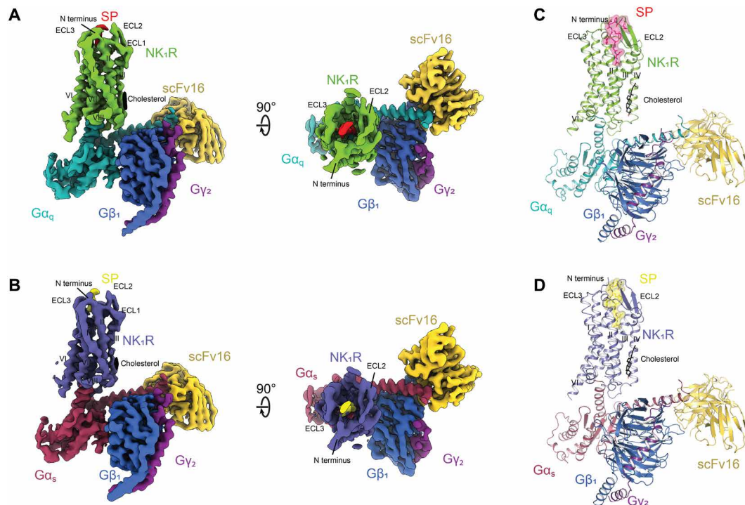
Fig. 1. Cryo-EM structures of NK 1 R:SP:G q :scFv16 and NK 1 R:SP:G s :scFv16. (A) Cryo-EM map of the NK 1 R:SP:G q :scFv16 complex resolved to 2.71 Å (FSC 0.143) as viewed from the side and from the top. (B) Cryo-EM map of the NK 1 R:SP:G s :scFv16 complex resolved to 2.87 Å (FSC 0.143) as viewed from the side and from the top. (C) Molecular model of the NK 1 R:SP:G q :scFv16 complex with SP and cholesterol shown in stick representation. (D) Molecular model of the NK 1 R:SP:G s :scFv16 complex with SP and cholesterol shown in stick representation.
