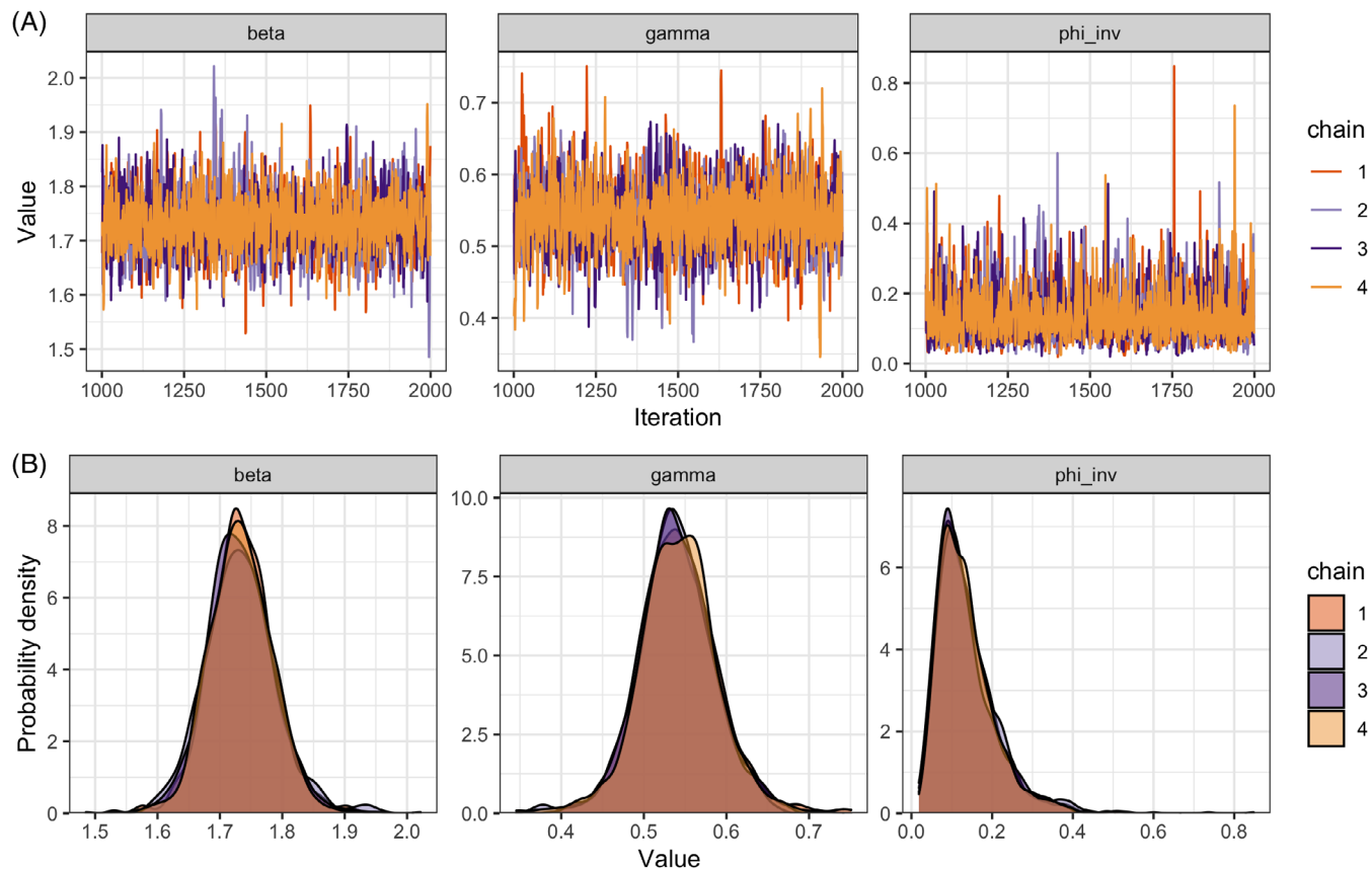
FIGURE 6 A, Trace plot showing the value of each chain at each iteration (excluding warm-up) and B, marginal posterior densities for the transmission rate ( \beta or \beta ), the recovery rate ( \gamma or \gamma ) and the inverse dispersion parameter ( \phi_{\text{inv}} or 1/\phi ), separately for each of the four Markov chains [Colour figure can be viewed at wileyonlinelibrary.com ]
