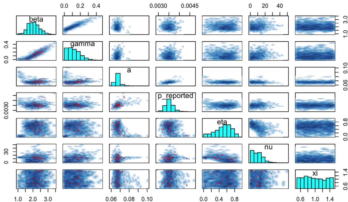
FIGURE 13 Pairs plot of all model parameters for the model incorporating control measures (model iteration #5) [Colour figure can be viewed at wileyonlinelibrary.com ]
