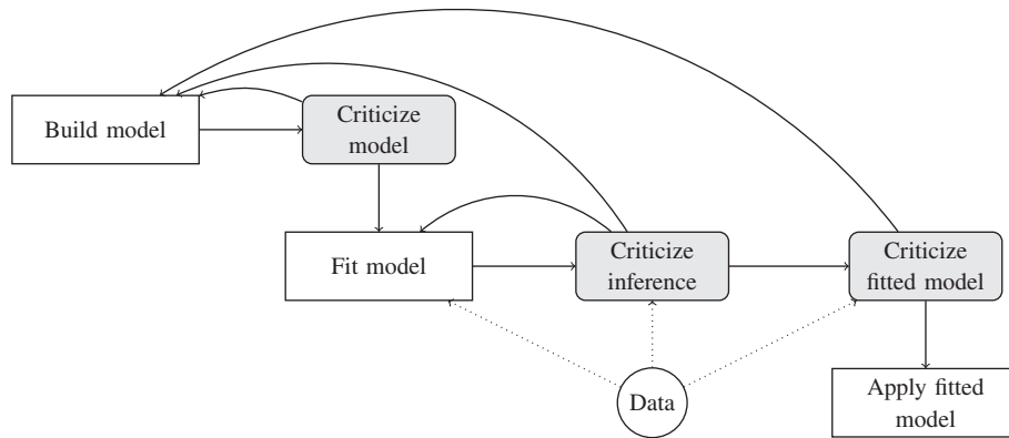
FIGURE 2 Model development as an iterative process
