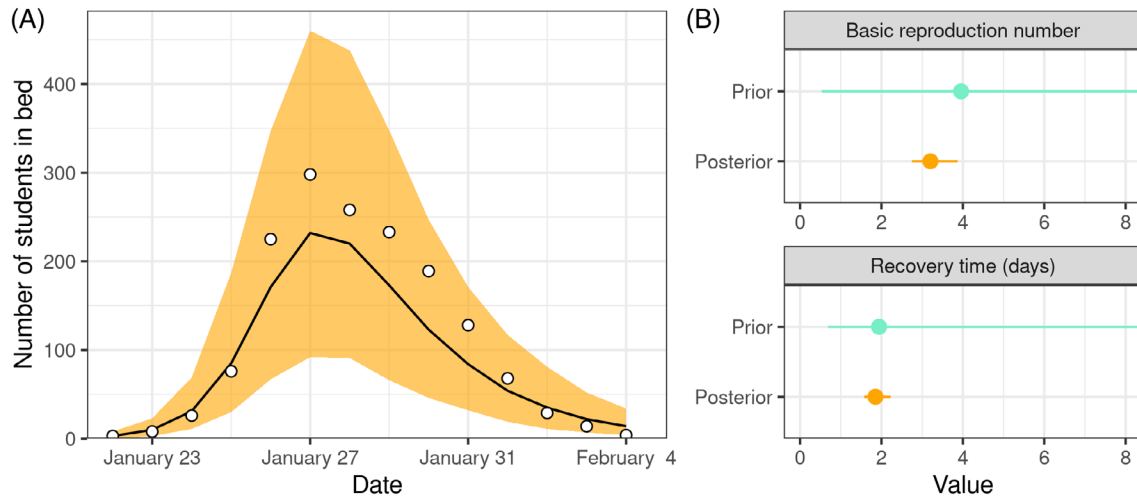
FIGURE 8 A, Posterior predictive check of the number of students in bed each day during an influenza A (H1N1) outbreak at a British boarding school. The line shows the median and the orange area the 90% prediction interval. B, Prior and posterior predictive checks of the basic reproduction number R_0 and of the recovery time (both truncated at 8). The dot shows the median posterior and the line shows the 95% credible interval [Colour figure can be viewed at wileyonlinelibrary.com ]
