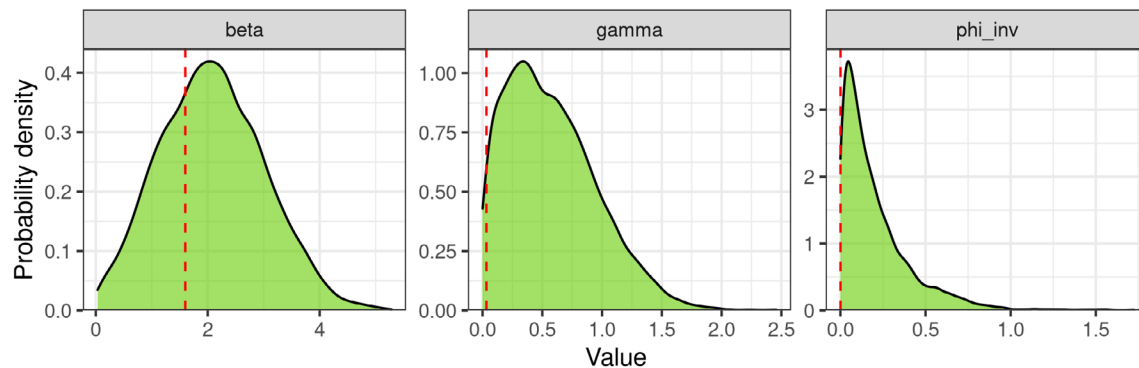
FIGURE 7 Marginal posterior densities for the transmission rate ( \beta or \beta ), the recovery rate ( \gamma or \gamma ) and the inverse dispersion parameter ( \phi_{\text{inv}} or 1/\phi ) obtained when fitting the model to simulated data. The red dashed lines show the fixed parameter values used for simulating the data [Colour figure can be viewed at wileyonlinelibrary.com ]
