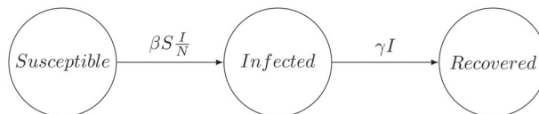
FIGURE 4 Diagram of the classic susceptible-infectious-recovered compartmental model
