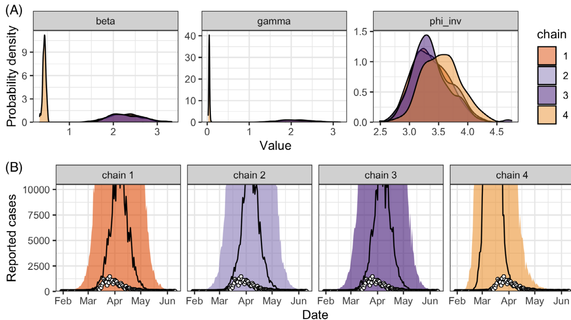
FIGURE 10 A, Posterior distributions of the model parameters (the transmission rate \beta , the recovery rate \gamma and the inverse dispersion parameter 1/\phi ) and B, chain-by-chain posterior predictive check of the number of reported cases for the simple SIR model (model iteration #1) applied to data on the SARS-CoV-2 epidemic in Switzerland (white circles). SARS-CoV-2, severe acute respiratory syndrome coronavirus 2; SIR, susceptible-infected-recovered [Colour figure can be viewed at wileyonlinelibrary.com ]
