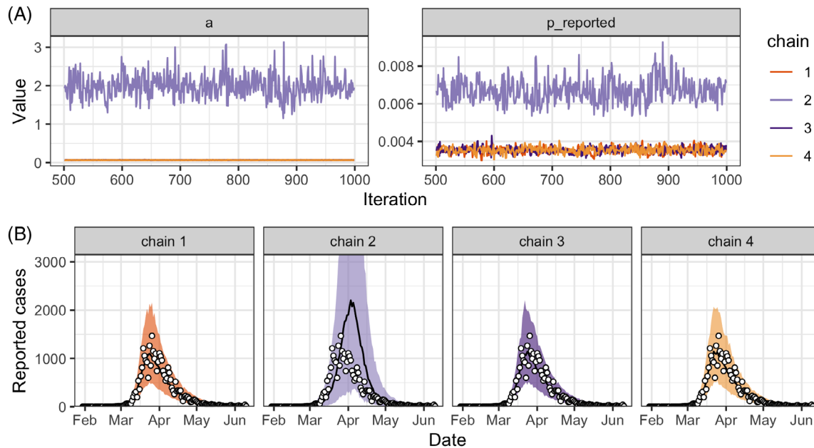
FIGURE 12 A, Trace plot for two of the model parameters (the incubation rate a and the reporting rate p_r —the other parameters are not shown) and B, posterior predictive check of the number of reported cases for the SEIR model with underreporting (model iteration #3) applied to data on the SARS-CoV-2 epidemic in Switzerland (white circles). SARS-CoV-2, severe acute respiratory syndrome coronavirus 2 [Colour figure can be viewed at wileyonlinelibrary.com ]
