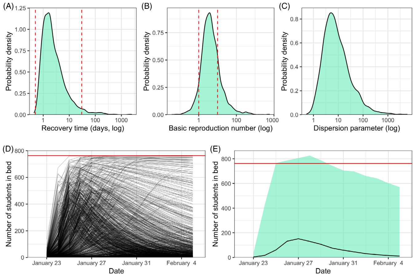
FIGURE 5 Prior predictive checks for (A) the recovery time ( 1/\gamma ), (B) the basic reproduction number \mathcal{R}_0 ( \beta/\gamma ), (C) the dispersion parameter ( \phi ), (D) a set of 1000 epidemic trajectories (each line is a unique simulated trajectory), and (E) the range in the numbers of students in bed each day (the line is the median and the light teal area is the 95% central range). All these quantities are sampled from the prior distributions of the parameters. The dashed red lines correspond to weak bounds from our domain knowledge where available: The recovery time is expected to last between 0.5 and 30 days, \mathcal{R}_0 cannot be lower than 1 or higher than 10. The plain horizontal red line shows the population size (763) [Colour figure can be viewed at wileyonlinelibrary.com ]
