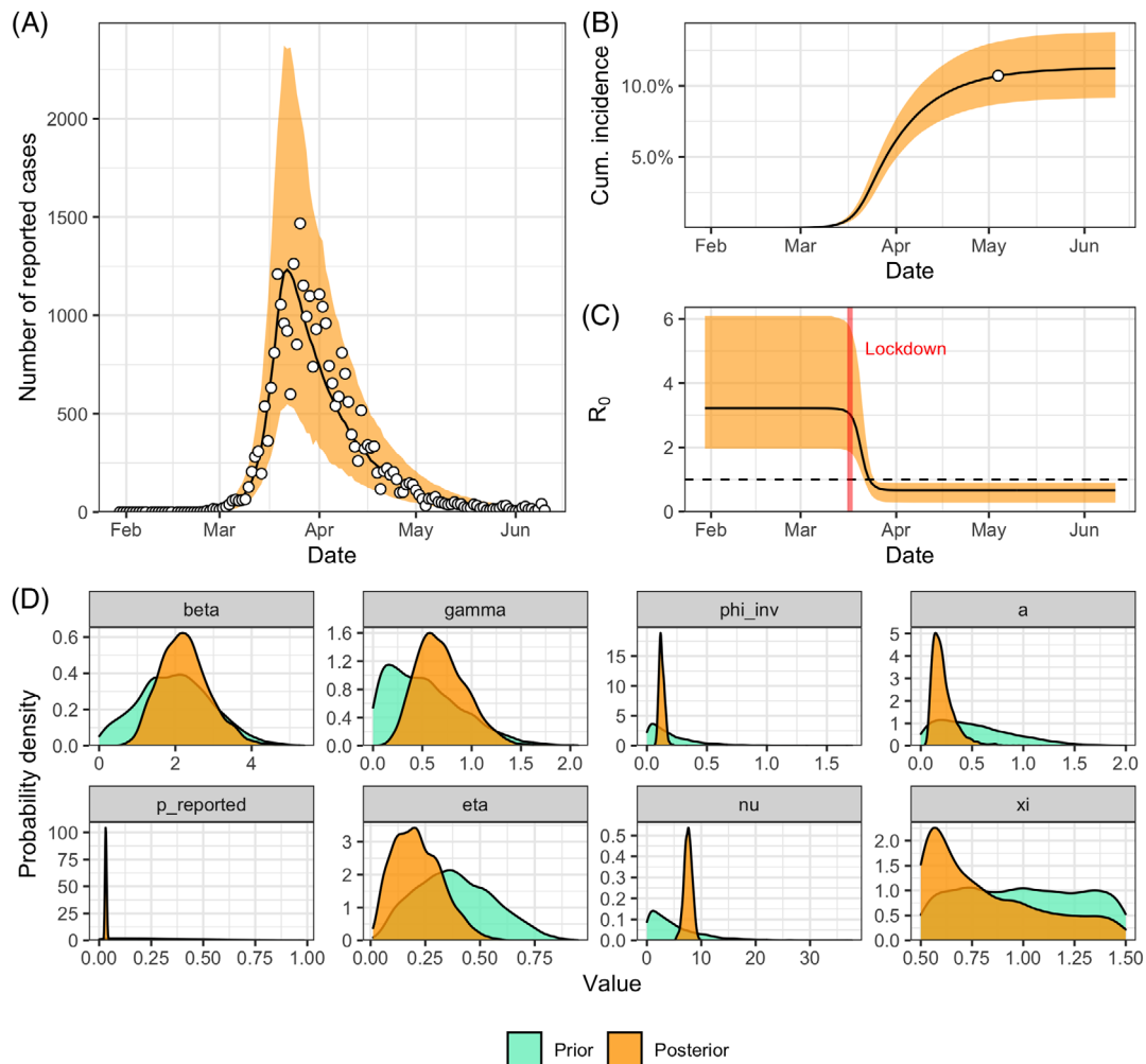
FIGURE 14 (A) Posterior predictive check of the number of reported cases and (B) of the cumulative incidence for the SEIR model including the effect of control measures and fitted to both reported cases and seroprevalence data (model iteration #7; white circles show data on reported cases in panel A and seroprevalence data in panel B). (C) Posterior distribution of the forcing function f that models the reduction in transmission after the introduction of lockdown measures. (D) Prior and posterior distributions of the parameters of model iteration #7 [Colour figure can be viewed at wileyonlinelibrary.com ]
