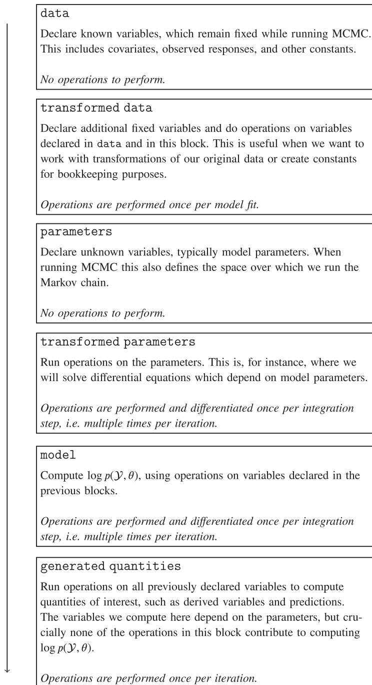
FIGURE 1 Coding blocks in a Stan file. The operations in certain blocks are performed multiple times and in some cases differentiated; as a result, the computational cost of fitting the model is dominated by the transformed parameters and model blocks. Not shown is the functions block, which defines functions that can be called in any of the operative blocks
