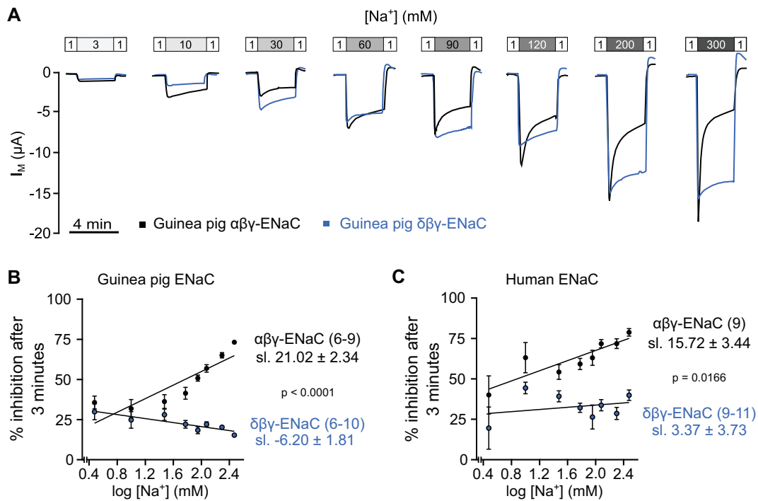
Fig. 8. The reduced sodium self-inhibition of human and guinea pig \delta\beta\gamma -ENaC generates increased activity at high extracellular Na + concentrations. (A) Representative transmembrane current ( I_M ) traces of guinea pig \alpha\beta\gamma - and \delta\beta\gamma -ENaC at different extracellular Na + concentrations ([Na + ]). Recordings of a given extracellular [Na + ] were performed in individual oocytes. The perfusion speed was 16 ml/min. (B, C) The percentage of sodium self-inhibition for guinea pig and human ENaC expressing oocytes plotted against logarithmic transformations of concentrations of extracellular [Na + ]. SSI was calculated as (\Delta I_M \text{ peak} - \Delta I_M \text{ 3 min}) / \Delta I_M \text{ peak} \times 100 , where \Delta I_M \text{ peak} = I_M under X mM [Na + ] peak – initial I_M under 1 mM [Na + ], and \Delta I_M \text{ 3 min} = I_M after 3 min under X mM [Na + ] – initial I_M under 1 mM [Na + ]. Slopes (sl.) were derived from linear regressions and P values, derived from ANCOVA, demonstrate the difference between slopes. Numbers in parentheses indicate (n).
